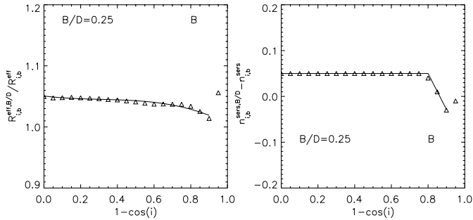
Fig. 5. As in Fig. 4, but for the derived effective radius R_{i,b}^{eff,B/D} (Left) and for the derived Sérsic indices (Right) of decomposed exponential bulges. The effects on Sérsic indices are represented as differences between the measured Sérsic index of decomposed and single bulges, n_{i,b}^{Sérsic,B/D} and n_{i,b}^{Sérsic} , respectively.
