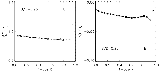
Fig. 4. Left: projection effects corr^{proj,B/D} on the derived scale-length of decomposed disks for B/D = 0.25 . The symbols represent the measurements while the solid lines are polynomial fits to the measurements. The plots represent the ratio between the intrinsic scale-lengths of decomposed and single disks, R_{i,d}^{B/D} and R_{i,d} , respectively, as a function of inclination ( 1 - \cos(i) ), for the B-band. An exponential (disk) plus a variable index Sérsic (bulge) distribution were used for image decomposition. Right: as in the left panel, but for the derived bulge-to-disk ratios, B/D . The effects are represented as differences between the intrinsic B/D of decomposed disks and bulges and those of single disks and bulges.
