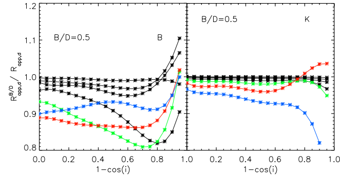
Fig. C.1. Dust effects ( corr^{B/D} - corr^{proj,B/D} ) on the derived scale-length of decomposed disks for B/D = 0.5 . The solid lines are polynomial fits to the measurements. The plots represent the ratio between the apparent scale-lengths of decomposed and single disks, R_{app,d}^{B/D} and R_{app,d} , respectively, as a function of inclination ( 1 - \cos(i) ), for the B and K optical bands. An exponential (disk) plus a variable index Sérsic (bulge) distribution were used for image decomposition. The black curves are plotted for \tau_B^f = 0.1, 0.3, 0.5, 1.0 , while the other curves correspond to \tau_B^f = 2.0 (green), 4.0 (red) and 8.0 (blue).
