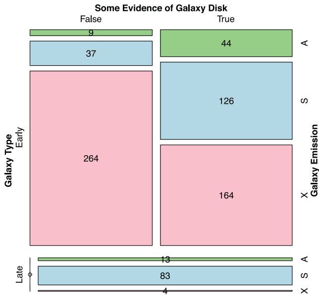
Figure A1. Mosaic plot of the data contained in Table A2. The contingency ordering is: type–disc–emission, where cell colouring is according to the emission contingency.
