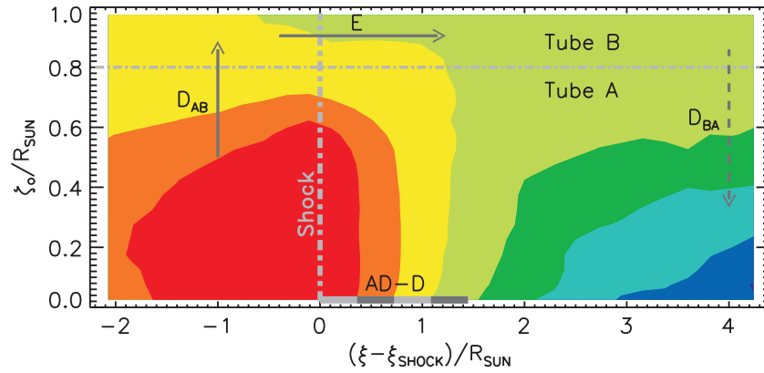
Figure 2. Map of the time-integrated distribution of >7 MeV protons on the \xi - \zeta_o plane in the shock frame. Red shows the highest density of the accelerated particles. Each following color level indicates one e -fold decline with respect to the previous one. The diffusion coefficient jump between the tubes is X = 50 . Perpendicular diffusion is energy dependent: D_{\perp}(E) = 0.04D_{\parallel}(E) . The integration time is 30 minutes.
