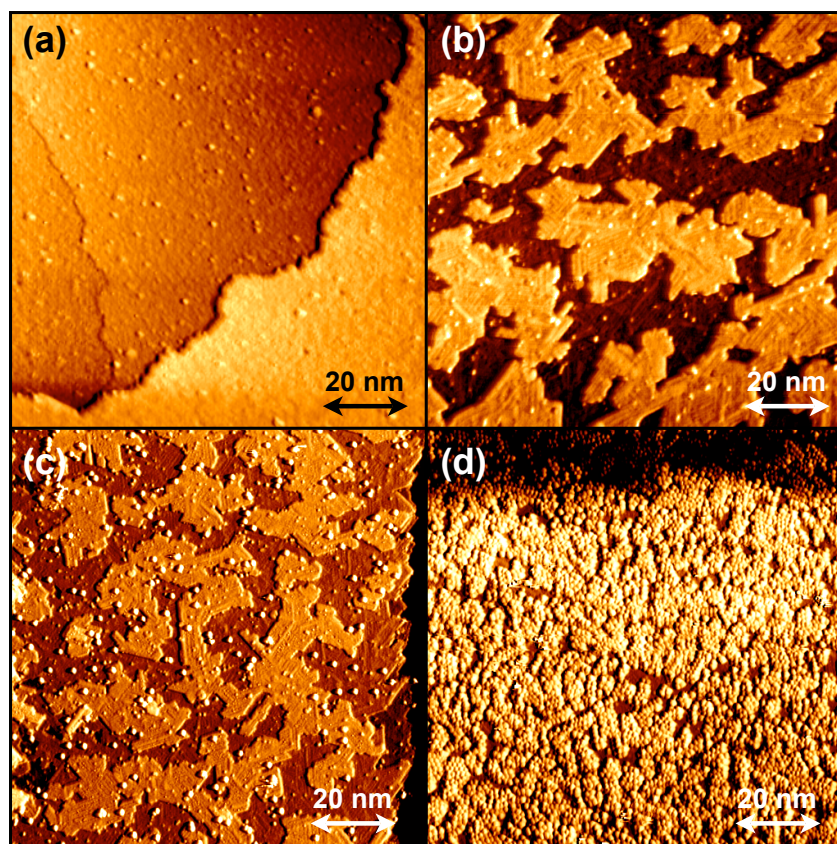
Figure 1. (a); A 100\text{ nm}\times 100\text{ nm} image of a clean Al-Pd-Mn surface, (b); A 100\text{ nm}\times 100\text{ nm} image of the 4.5 \pm 0.1\text{ ML} Cu layer deposited on the Al-Pd-Mn surface. The lighter rows have previously been identified as strain-related defects [19], the white spots are contamination, (c); 0.025\text{ ML} \text{C}_{60} adsorbed atop the Cu layer, showing an absence of island formation, (d); 0.8\text{ ML} \text{C}_{60} adsorbed atop the Cu layer, showing some evidence of orientation of rows of \text{C}_{60} .
