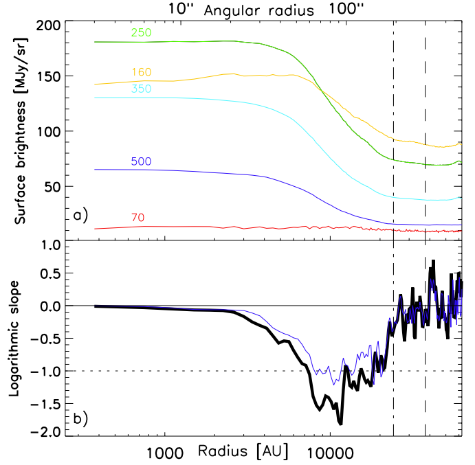
Fig. A.1. a) Circularly averaged radial surface brightness profiles of B68 at 70, 160, 250, 350, 500 \mu\text{m} derived from Herschel /SPIRE and PACS data (after adding Planck offsets). b) Logarithmic slopes of the circularly averaged column density profile (solid black curve) and 500 \mu\text{m} intensity profile (solid blue curve) of B68 as a function of radius. The horizontal dotted line is the logarithmic slope s = -1 expected for the column density profile of a core with a \rho \propto r^{-2} density profile. The vertical dashed line marks the integration upper bound adopted when integrating the right-hand side of Eq. (2) to perform the Abel reconstruction of the density and temperature profiles (see Sect. 3). The vertical dot-dashed line shows the radius of the footprint automatically derived for B68 by the getsources source-finding algorithm.
