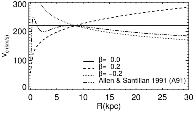
Fig. 2. Rotation curves of Eq. (1) with different values for \beta : flat \beta = 0 (solid line), raising \beta = 0.2 (dashed line), and decreasing \beta = -0.2 (dotted line) rotations curves. The dotted-dashed line shows the rotation curve of the Allen & Santillan (1991) model (A91).
