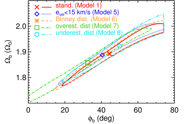
Fig. 16. Two-dimensional (marginalised over \beta ) likelihood in the \phi_b - \Omega_b space for different cases of RAVE data. The different lines show the 1\sigma confidence regions and the different symbols are the two dimensional maxima of the likelihood.
