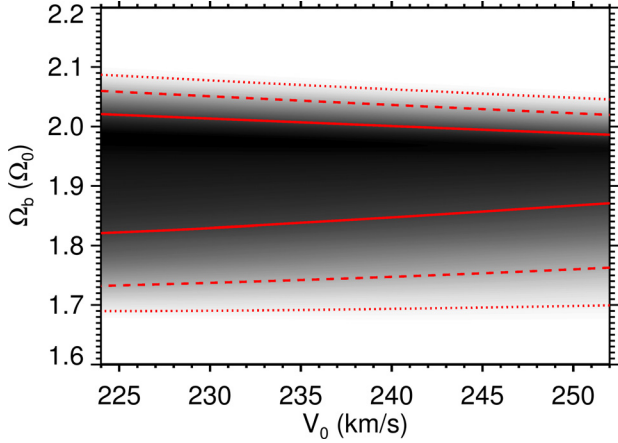
Fig. 14. Two-dimensional (marginalised over the other parameters) likelihood function in the v_0 - \Omega_b plane for the RAVE data.
