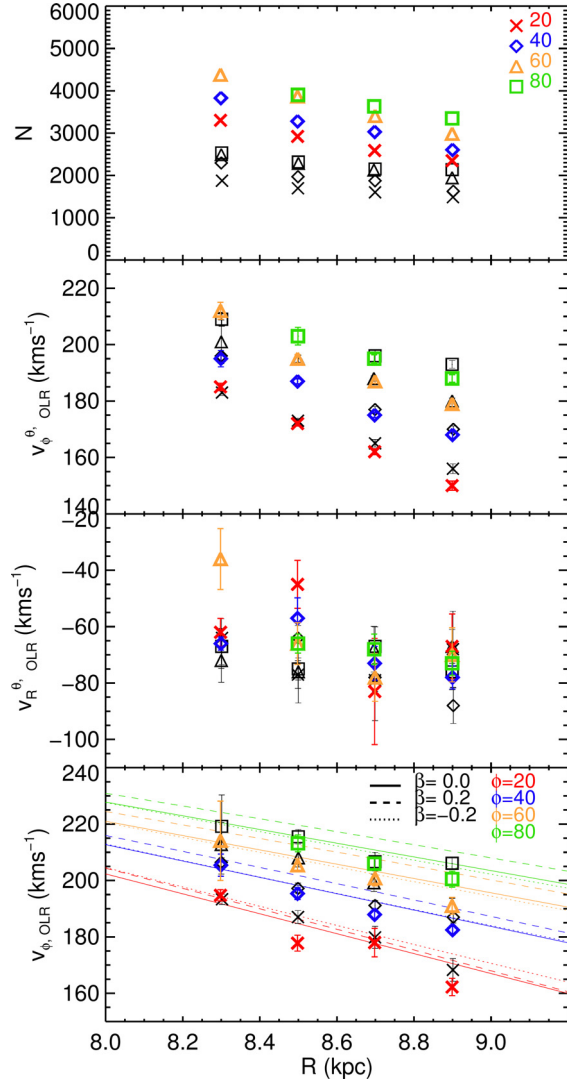
Fig. B.2. Several measurements for the bands at different bar angles as in Fig. 6 when we add RAVE errors (black symbols) and when we also allow for contamination from stars at other distances (colour symbols).
