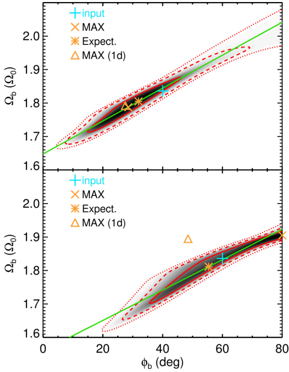
Fig. 7. Two-dimensional marginalised likelihood (over the parameter \beta ) of the model parameters for the simulated bands at 40 deg ( top ) and 60 deg ( bottom ). Solid, dashed and dotted red lines show the 1\sigma , 2\sigma and 3\sigma confidence regions, respectively. The input parameters of the simulation are shown with a light blue cross. The maximum and the expected value of the two-dimensional pdf are indicated with an orange cross and asterisk, respectively. The orange triangle is the maximum of the one-dimensional marginalised pdf's.
