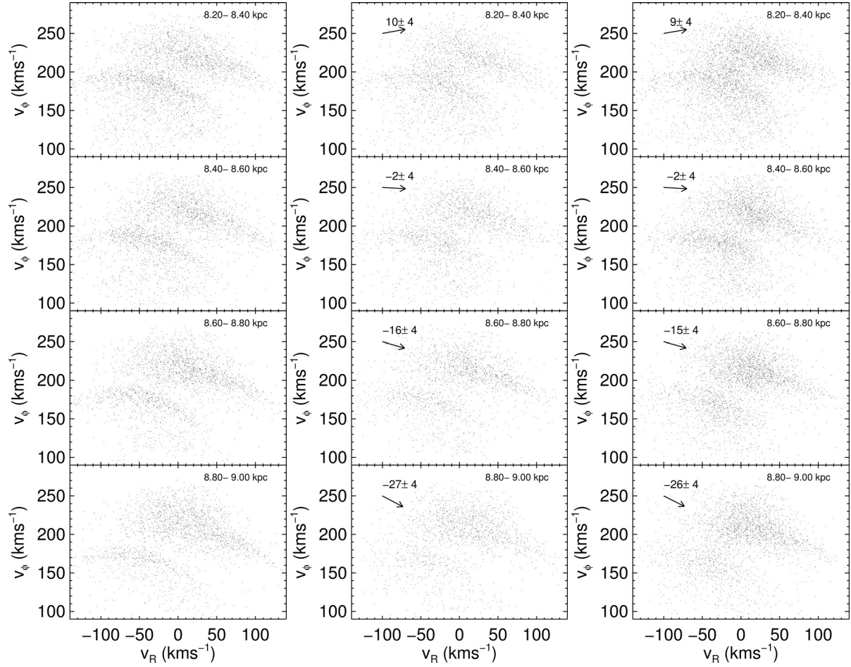
Fig. B.1. Scatter plot of the velocities in bins in radius as indicated in the top right part of the panels for the band at 40 deg with no error convolution ( left ), with RAVE error convolution ( middle ) and with error convolution and allowing contamination from stars at different distances ( right , see text). The numbers and the errors in the top left part of the panels are the median and dispersion of the direction of the transverse movement, taken as a counterclockwise angle with respect to the v_R axis. The arrows indicate this median direction.
