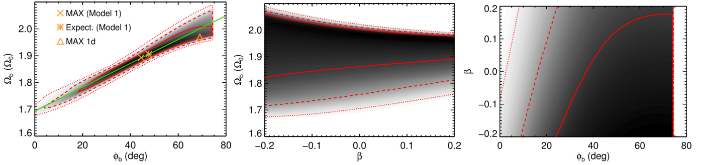
Fig. 12. Two-dimensional marginalised likelihoods (over the 3rd parameter) for the model parameters for the RAVE data. Solid, dashed and dotted red lines show the 1\sigma , 2\sigma and 3\sigma confidence regions, respectively. In the left panel the maximum and the expected value of the two-dimensional pdf are indicated with an orange cross and asterisk, respectively. The orange triangle is the maximum of the one-dimensional marginalised pdf's.
