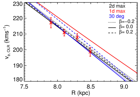
Fig. 11. Position of the v_{\phi, \text{OLR}} as a function of R for the band at \phi_b + 6 deg for the RAVE data. Several fits from Table 3 (see text) are overplotted.
