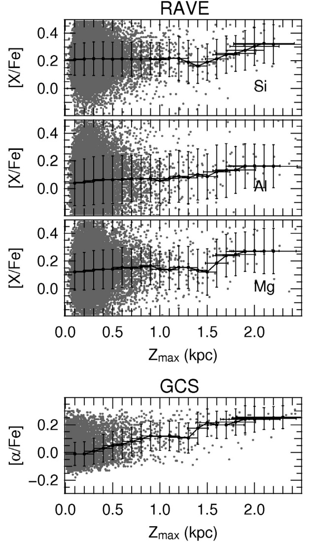
Fig. 7. Relative abundances [Mg/Fe], [Al/Fe], and [Si/Fe] for RAVE ( top ), and [\alpha/\text{Fe}] for GCS ( bottom ) as a function of Z_{\text{max}} . Horizontal and vertical error bars are defined as in Fig. 5.
