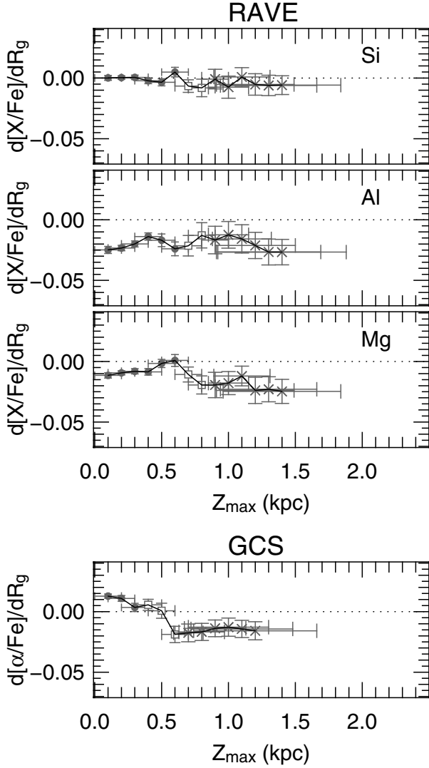
Fig. 6. Gradients for the RAVE relative abundances [Mg/Fe], [Al/Fe], and [Si/Fe] for RAVE ( top ), and [\alpha/\text{Fe}] for GCS ( bottom ) as a function of Z_{\text{max}} . Horizontal and vertical error bars are defined as in Fig. 4.
