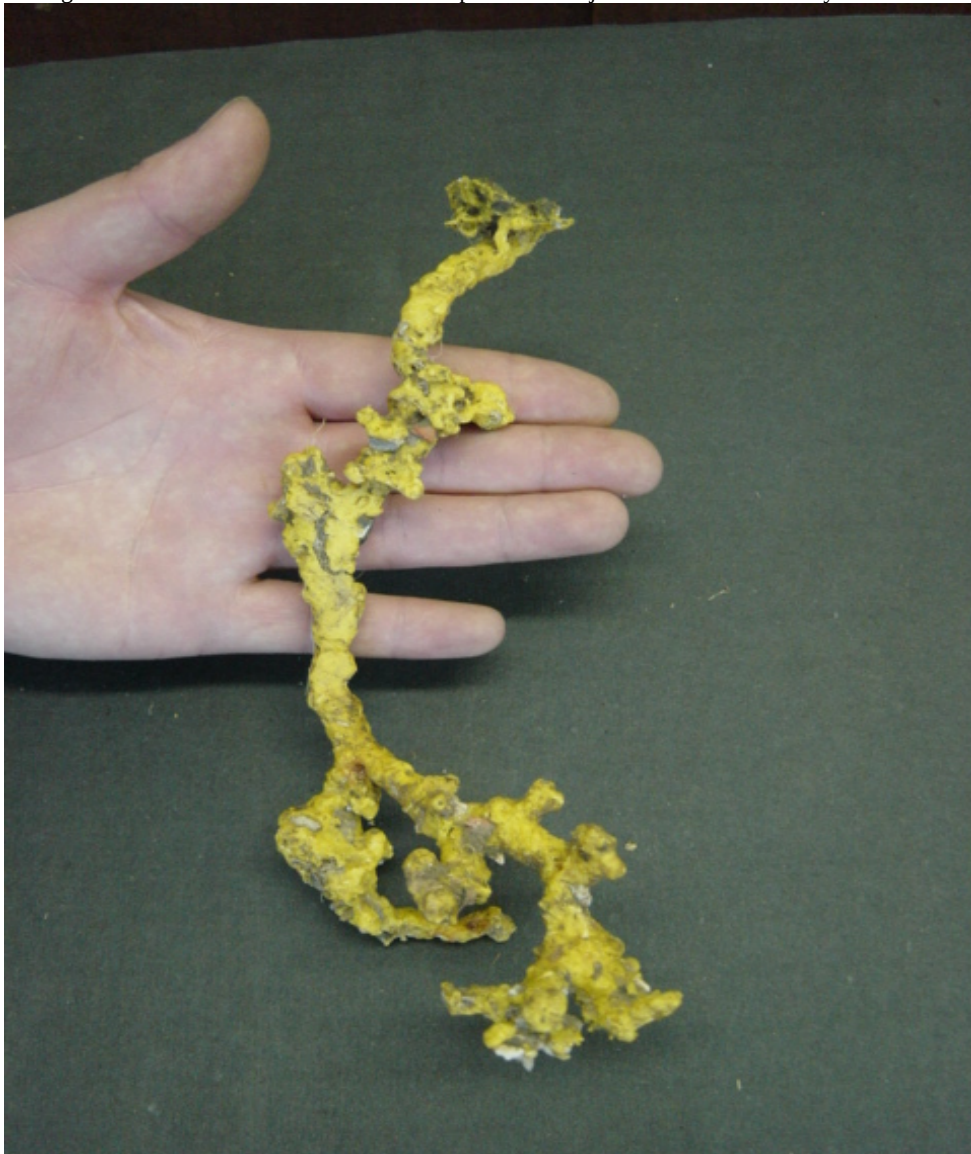
Fig. 5. Example of an extracted polyurethane cast of a Lumbricus terrestris burrow from Preston Cemetery, showing multiple branches (total depth = 0.2 m)
