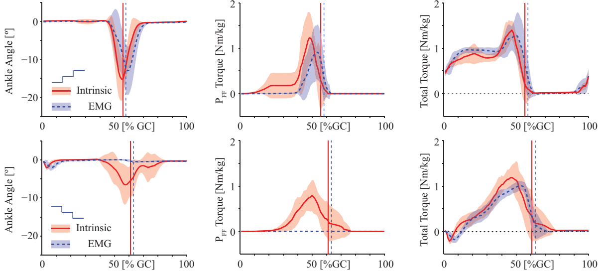
Figure 2 – Ankle-Angle, PFF torque, and total estimated torque over the gait cycle. During stair ascent (top row) the participant was able to reliably activate his gastrocnemius muscle to modulate the power provided by the powered ankle-foot prosthesis during PP phase. He could thereby achieve the same ankle-angle and overall torque profile as with the intrinsic controller. Maximal PFF torque was higher for the intrinsic controller; however, this was not reflected in the overall torque profile. Importantly, as indicated in the bottom row, minimizing gastrocnemius activity prevented the prosthesis from inadvertently providing power during stair descent. This was not the case while walking with the intrinsic controller as indicated by the larger ankle-angle and PFF torque.
