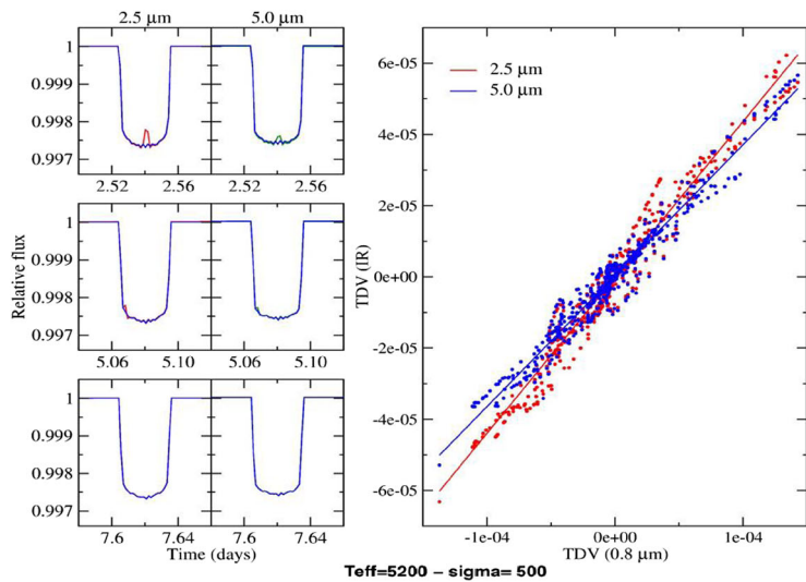
Teff=5200 - sigma= 500
