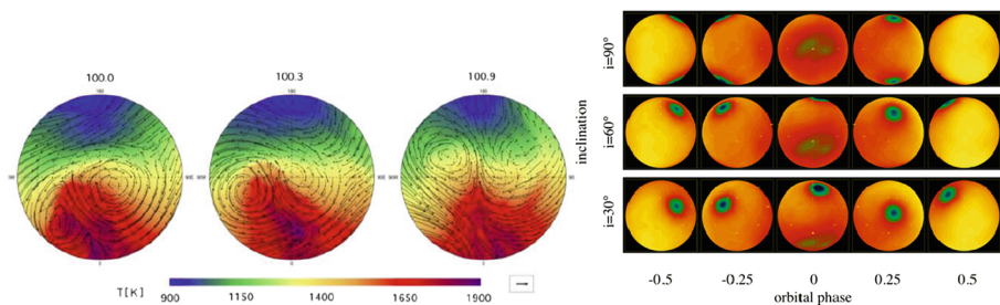
Fig. 7 Left: Giant storms on a synchronized, gaseous planet. Wind vectors superimposed on temperature map over approximately one planet rotation period, viewed from the north pole. Synchronized planets experience intense irradiation from the host star (at \text{lon}=0 point), exciting large-amplitude planetary waves and active storms that move off to the night side (top half in each frame). The storms dissipate and regenerate with a distinct period of a few planet rotations [41, 42]. Other dynamically-induced periodicities are present on synchronized planets. The periodicities can be used to distinguish synchronized and unsynchronized planets, among other things. Right: Simulated phase variations for a hot-Jupiter with different inclinations [129]
