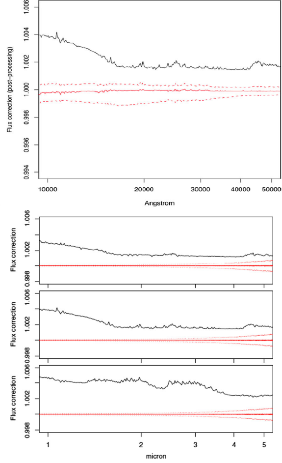
Teff=5200 - sigma= 500
