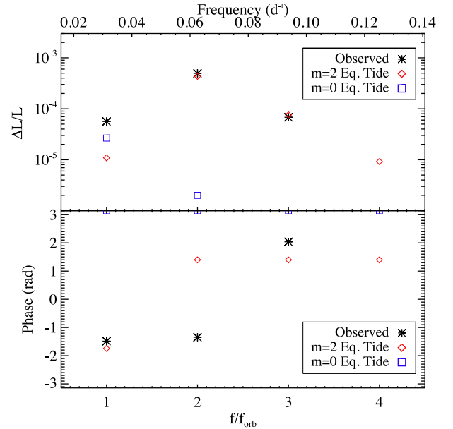
Figure 12. Top: observed luminosity fluctuations and luminosity fluctuations due to the equilibrium tidal distortion (calculated using Von Zeipel's theorem) as a function of the orbital harmonic f/f_{\text{orb}} . Bottom: observed cosine phase of the luminosity fluctuations and the expected phase for the equilibrium tide. Although the observed oscillation amplitude at 2f_{\text{orb}} is near the expected equilibrium tide amplitude, it is out of phase from the expected equilibrium tide phase.
