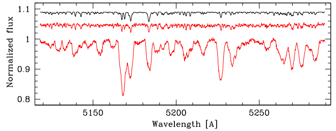
Figure 5. Disentangled spectra of the components in the binary system HD 183648 (lower two spectra) in the spectral region centred on the Mg I triplet \lambda\lambda 5167–5184 Å. For comparison, the top curve is a synthetic spectrum of a star with atmospheric parameters of the secondary (cf. Table 7), rotationally broadened with v_{\text{rot}} \sin i_{\text{rot}} = 26 \text{ km s}^{-1} and diluted by a factor of 20.
