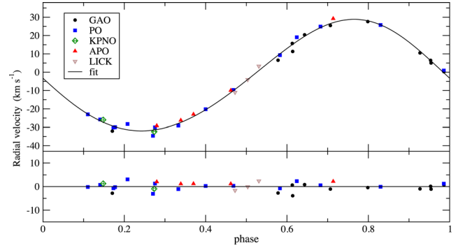
Figure 4. The observed radial velocities and the best-fitting RV solution for the \dot{V}_\gamma \equiv 0 case (solid line). The residuals of the fit are shown in the lower panel.
