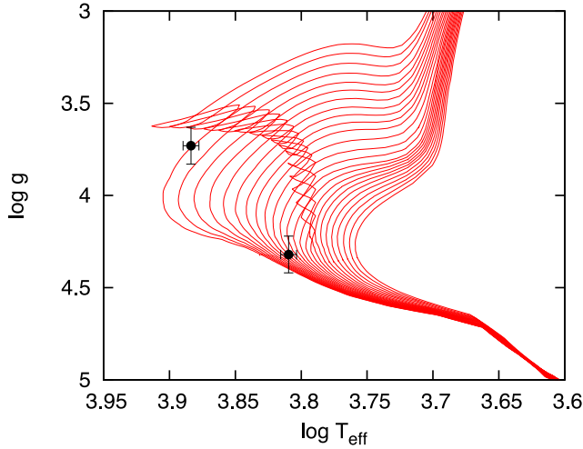
Figure 3. The position of the two components on the T_{\text{eff}} - \log g evolution tracks with [Fe/H] = -0.5 metallicity.
