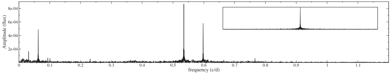
Figure 11. The pulsational amplitude spectrum of 17 quarters of long cadence data for HD 183648. The inset shows the spectral window.
