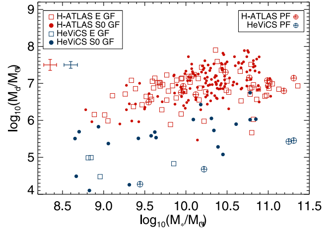
Figure 10. MAGPHYS dust mass plotted as a function of stellar mass. HeViCS (blue points) and H-ATLAS (red points) samples are shown, where galaxies are subdivided into E (red squares for H-ATLAS and blue squares for HeViCS) and S0 (red dots for H-ATLAS and blue dots for HeViCS) classifications. Galaxies with PF are circled crosses in the samples' respective colours. Error bars give 1\sigma to each side of the PDF, in the same colours as their respective samples.
