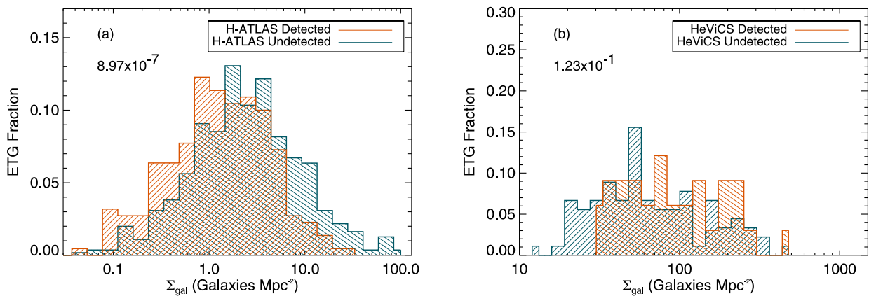
Figure 5. Left-hand panel: normalized distributions of submm detected (orange histogram) and submm undetected (blue histogram) ETG in H-ATLAS. Right-hand panel: distributions of submm detected (orange histogram) and submm undetected (blue histogram) ETG in HeViCS. KS probabilities for whether the presented samples are drawn from the same distribution are shown in the top left of the plots.
