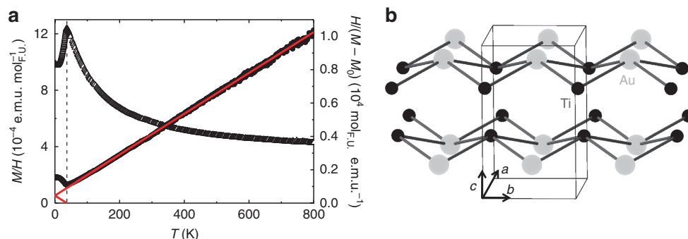
Figure 1 | Temperature-dependent magnetization of TiAu. (a) Left axis: zero-field-cooled magnetic susceptibility as a function of temperature for \mu_0 H = 0.1 T applied field (1 e.m.u. = 10 \text{ A cm}^{-2} ). Right axis: inverse susceptibility H/M along with a Curie–Weiss-like fit (solid line), with \theta \approx -37 K (marked by a dashed line). (b) The crystal structure of TiAu with Ti (small) and Au (large) atoms, and the orthorhombic unit cell outlined in thin black lines. The arrows identify the crystallographic directions, marked by a , b and c axes.
