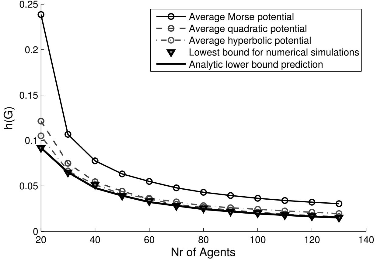
FIG. 5: Comparison of Cheeger constant obtained by the analytic expression simply based on the number of particles and that obtained through numerical simulations averaged over 100 runs with random initial conditions.
