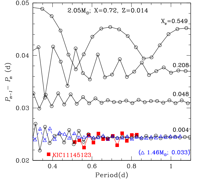
Figure 6. Period spacings of g modes ( P_{n-1} - P_n ) as a function of g-mode period for selected evolutionary stages of the 2.05- M_\odot model with (X, Z) = (0.72, 0.014) . The observed period spacings of KIC 11145123 are shown by filled squares. Also plotted (triangles) are period spacings of the best model of 1.46 M_\odot with (X, Z) = (0.65, 0.010) . This shows KIC 11145123 to be at the TAMS stage with core hydrogen heavily depleted.
