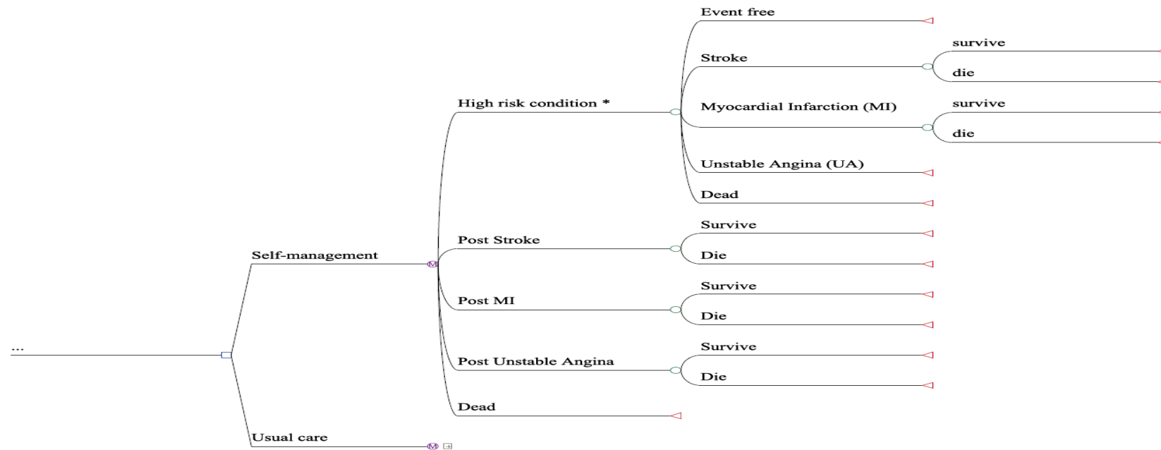
Figure 1 Markov model
