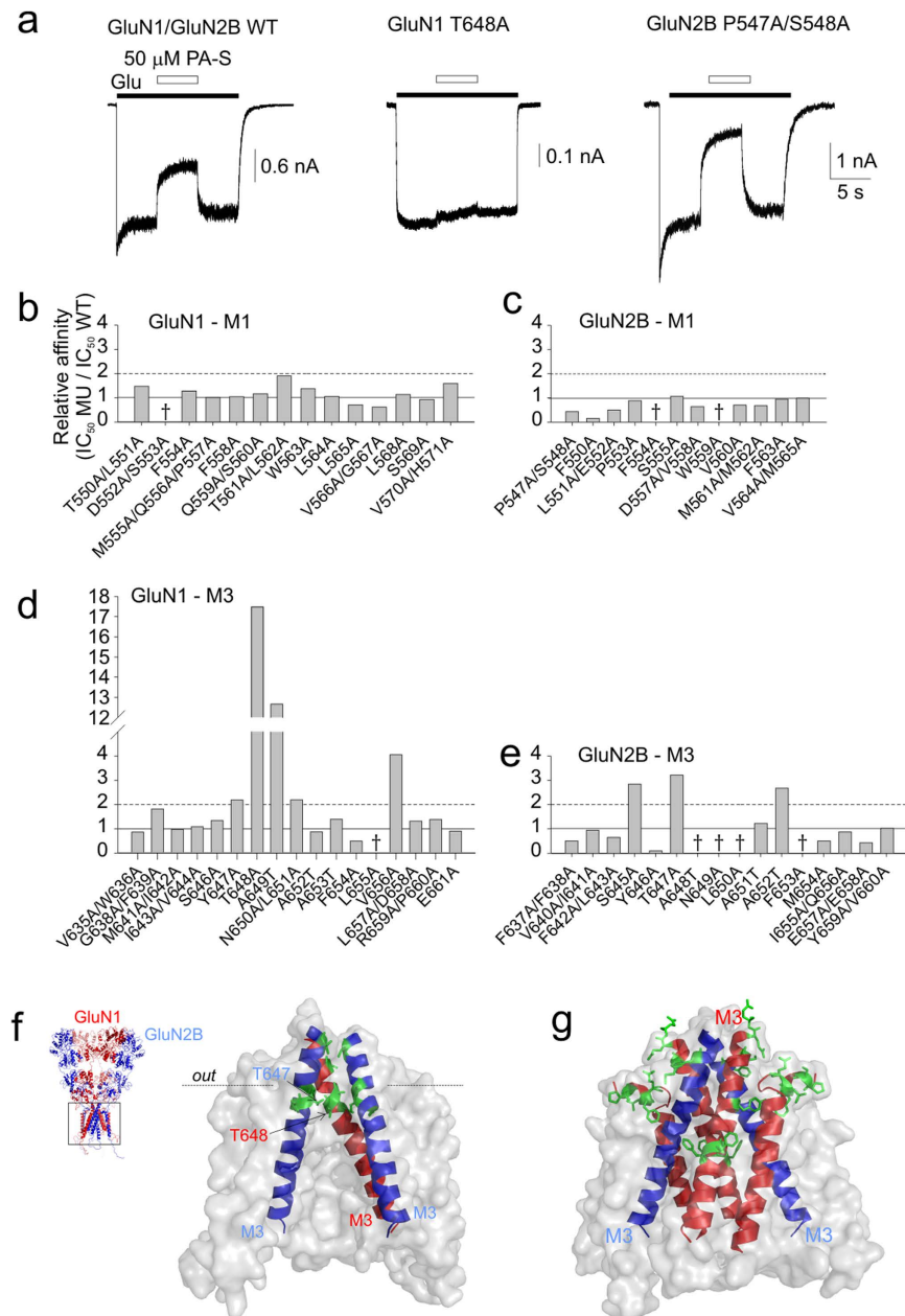
Figure 2. Mutations in the M1 and M3 regions of the GluN1 and GluN2B subunits alter the inhibitory potency of PA-S. (a) A representative response is shown for WT and mutated GluN1/GluN2B receptors. Responses mediated by GluN1(T648A)/GluN2B receptors were assessed as a difference between the current recorded in the presence of 1 mM Mg^{2+} (condition that abolished the spontaneous currents) and that recorded in the presence of 1 mM glutamate and 10 \mu M glycine. While the GluN1(T648A)/GluN2B receptors were only slightly affected by PA-S (50 \mu M) when compared to the WT receptor, the GluN1/GluN2B(P547A/S548A) receptors were more sensitive to the steroid. Graph of the relative PA-S affinity for NMDARs mutated in the M1 regions of GluN1 (b) and GluN2B (c) or mutated in the M3 regions of GluN1 (d) and GluN2B (e) are shown. Relative PA-S affinity was determined as the ratio of PA-S IC_{50} (Equation 1) determined for mutated receptors and the IC_{50} for the WT receptor (42 \mu M; n = 20 ). † indicates a non-responding mutation, i.e. a minimum of six GFP-positive cells responding to 1 mM glutamate application with currents <20 pA. (f) Amino acid residues whose mutations altered PA-S inhibition are depicted in a homology model of GluN1/GluN2B. For clarity, only the transmembrane region is shown. GluN1 is colored in light blue and GluN2B is colored in light red. Dashed line indicates the boundary between hydrophobic and hydrophilic regions of lipid as determined by the OPM database 63 . Residues whose mutation to alanine increased the IC_{50} for PA-S inhibition of GluN1/GluN2B receptor responses more than two-fold (to >84 \mu M) are highlighted in green. (g) Residues whose mutation to alanine decreased the IC_{50} for PA-S inhibition by half (to <21 \mu M) are highlighted in green.
