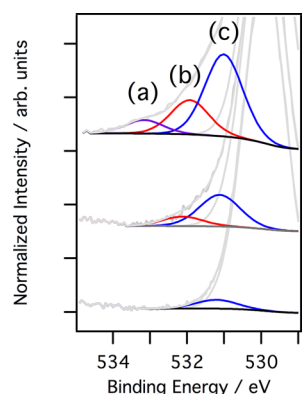
Figure 4. O 1s spectra, focusing on the peaks introduced after dosing PPA to the high binding energy side of the oxide peak. The blue curve (c) is assigned to Ti–O–P bonds following dissociation of the OH groups and the red curve (b) to the unbound phosphonyl P=O. At the 0.85 ML coverage a third peak is evident, marked by a purple line (a), which arises from undissociated P–OH.
