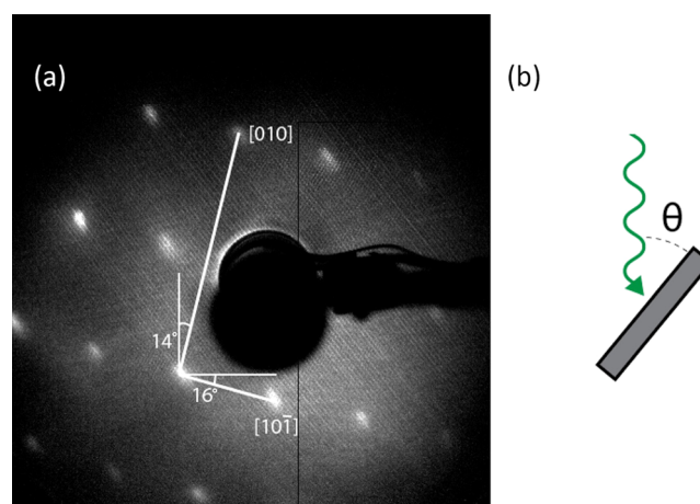
Figure 2. (a) 1 \times 1 LEED pattern obtained for anatase \text{TiO}_2(101) surface. The arrows show how the azimuthal angle is defined in the NEXAFS experiments described below. (b) Definition of the polar angle in the NEXAFS experiments.
