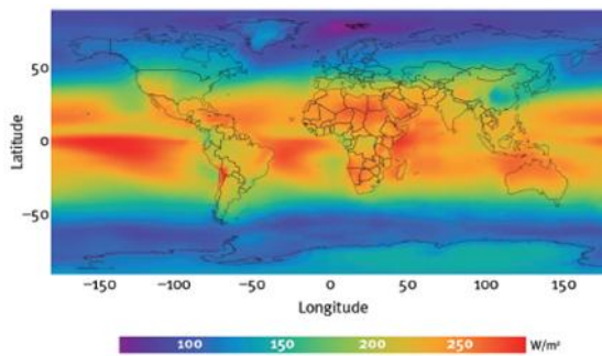
Figure 1. Distribution of annual average solar irradiance over the Earth's surface
