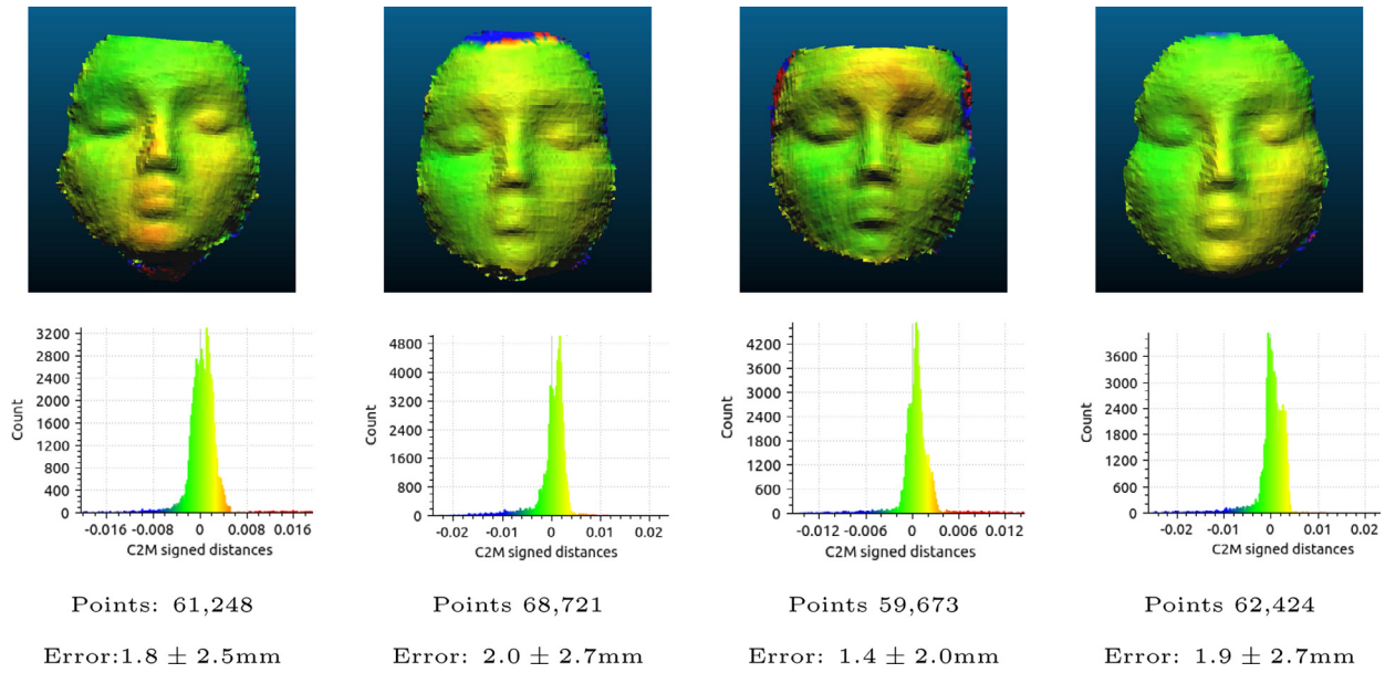
Fig. 8. Comparison between 3D reconstructions obtained using the proposed method. The images on the top represent the signed distance between the two reconstructions: the current reconstruction and a reference reconstruction. The histograms (on the bottom) are calculated with the number of points belonging to the reconstructed face (63,000 points on average) and clustered depending on their signed distance (in meters) to the reference scan. The average error for all the experiments is 1.7 \pm 2.4 mm.
