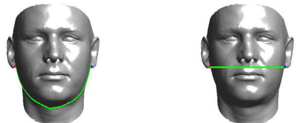
Fig. 11. Geodesic (left) and Euclidean (right) distance between two landmarks.
