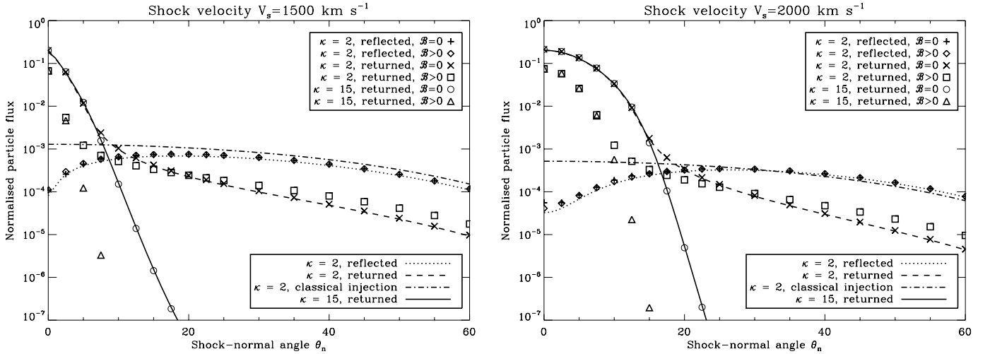
Fig. 6. Particle fluxes at the shock: curves represent numerical integration results, data points are results of Monte Carlo simulations. V_s = 1500 \text{ km s}^{-1} (left) and V_s = 2000 \text{ km s}^{-1} (right). Simulations without downstream propagation of particles are designated with \mathcal{B} = 0 , whereas simulations where particles isotropise through downstream scatterings are designated with \mathcal{B} > 0 . The flux differences for the reflected particles in the Monte Carlo simulations ( \diamond , + ) are due to statistical uncertainties. For comparison, we show the integrated flux of all particles that are faster than the classical injection threshold v > u_1 as a dash-dotted line. For \kappa = 15 , reflected particle fluxes and the classical comparison are too low to be visible.
