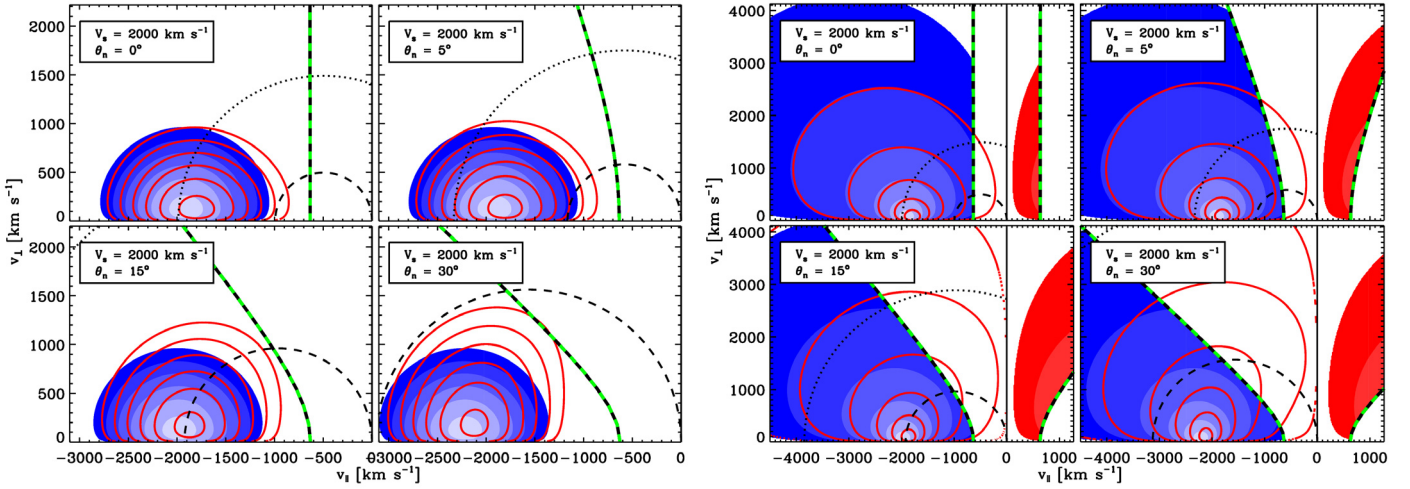
Fig. 5. Visualised transfer of quasi-thermal (left, \kappa = 15 ) and non-thermal (right, \kappa = 2 ) particle flux densities d\mathcal{F}/(dv_{\parallel} dv_{\perp}) across a shock of velocity V_s = 2000 \text{ km s}^{-1} with four different shock-normal angles. Blue contours depict the incident transmitting flux, red contours depict the reflected flux, and red solid contours the transmitted downstream flux at one magnitude intensity intervals. The black semicircles depict downstream speed thresholds for statistical return probabilities of 0% (dashed) and 25% (dotted), and the black-green dashed curve represents the reflection threshold.
