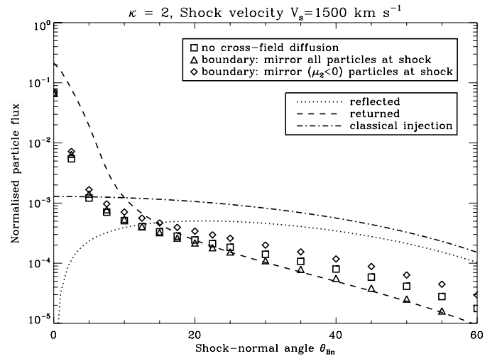
Fig. 7. Effect of downstream cross-field diffusion strength a_\perp = 0.1 on the injection efficiency for V_s = 1500 \text{ km s}^{-1} , \kappa = 2 , and different shock-normal angles. Curves (from numerical integration results) and results from simulations without cross-field diffusion (squares) are the same as in Fig. 6. Results for the two types of downstream cross-field diffusion (sets three and four) are shown as triangles and diamonds.
