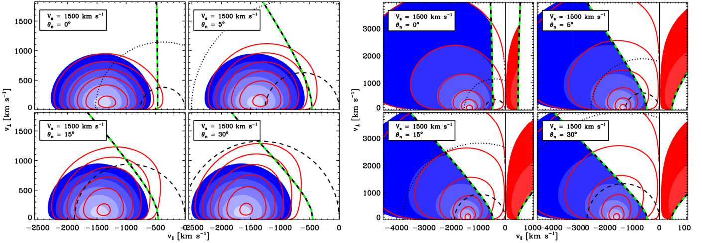
Fig. 4. Visualised transfer of quasi-thermal (left, \kappa = 15 ) and non-thermal (right, \kappa = 2 ) particle flux densities d\mathcal{F}/(dv_{\parallel} dv_{\perp}) across a shock of velocity V_s = 1500 \text{ km s}^{-1} with four different shock-normal angles. Blue contours depict the incident transmitting flux, red contours depict the reflected flux, and red solid contours the downstream transmitted flux at one magnitude intensity intervals. The black semicircles depict downstream speed thresholds for statistical return probabilities of 0% (dashed) and 25% (dotted), and the black-green dashed curve represents the reflection threshold.
