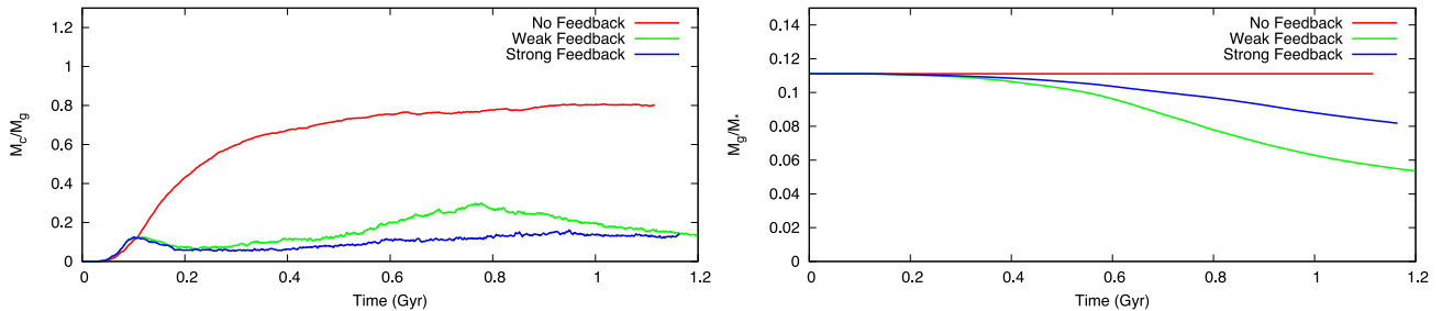
Figure 3. Left: evolution of the mass of clouds as a fraction of the total mass of gas particles (i.e. M_c/M_g ) in runs with and without feedback. In the no-feedback model, clouds continually accrete material. With feedback, gas is recycled and less mass is retained within the cloud. The peak at \sim 800 Myr in the weak-feedback run results from the build-up of massive clouds that are not properly disrupted by weak feedback. Right: evolution of the ratio of gas mass to stellar mass ( M_g/M_* ) in runs with and without feedback. Gas is depleted more rapidly with weak feedback likely because clouds are less disrupted. Gas is not depleted in the no-feedback run.
