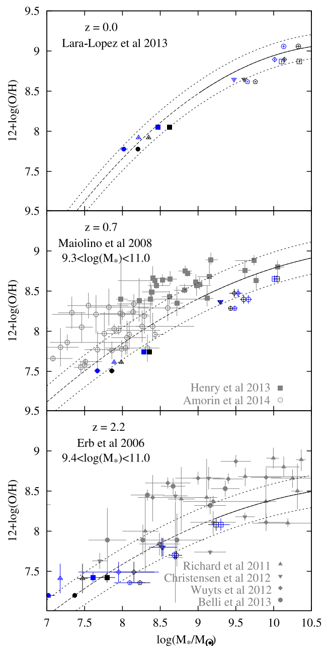
Figure 7. Oxygen abundance as function of stellar mass at three different redshifts. The blue and black points correspond to masses derived using the mass-to-light ratio in the B band and to true simulation values, respectively. The shape coding is the same as in Fig. 4. In the centre and bottom panels, we overplotted in grey some of the observational samples (indicated in the corresponding legends) which have the lowest mass system detected at intermediate and high- z . The black solid curves are the observational M – Z relations obtained by Lara-López et al. (2013, top panel), Maiolino et al. (2008, centre panel) and Erb et al. (2006, bottom panel). The dashed black lines give the low-mass extrapolation of these relations, while the dotted black ones give the scatter of 0.15, 0.20 and 0.20 dex, respectively. The limits in the centre and bottom panels indicate the corresponding stellar mass ranges for the samples of Maiolino et al. (2008) and Erb et al. (2006).
