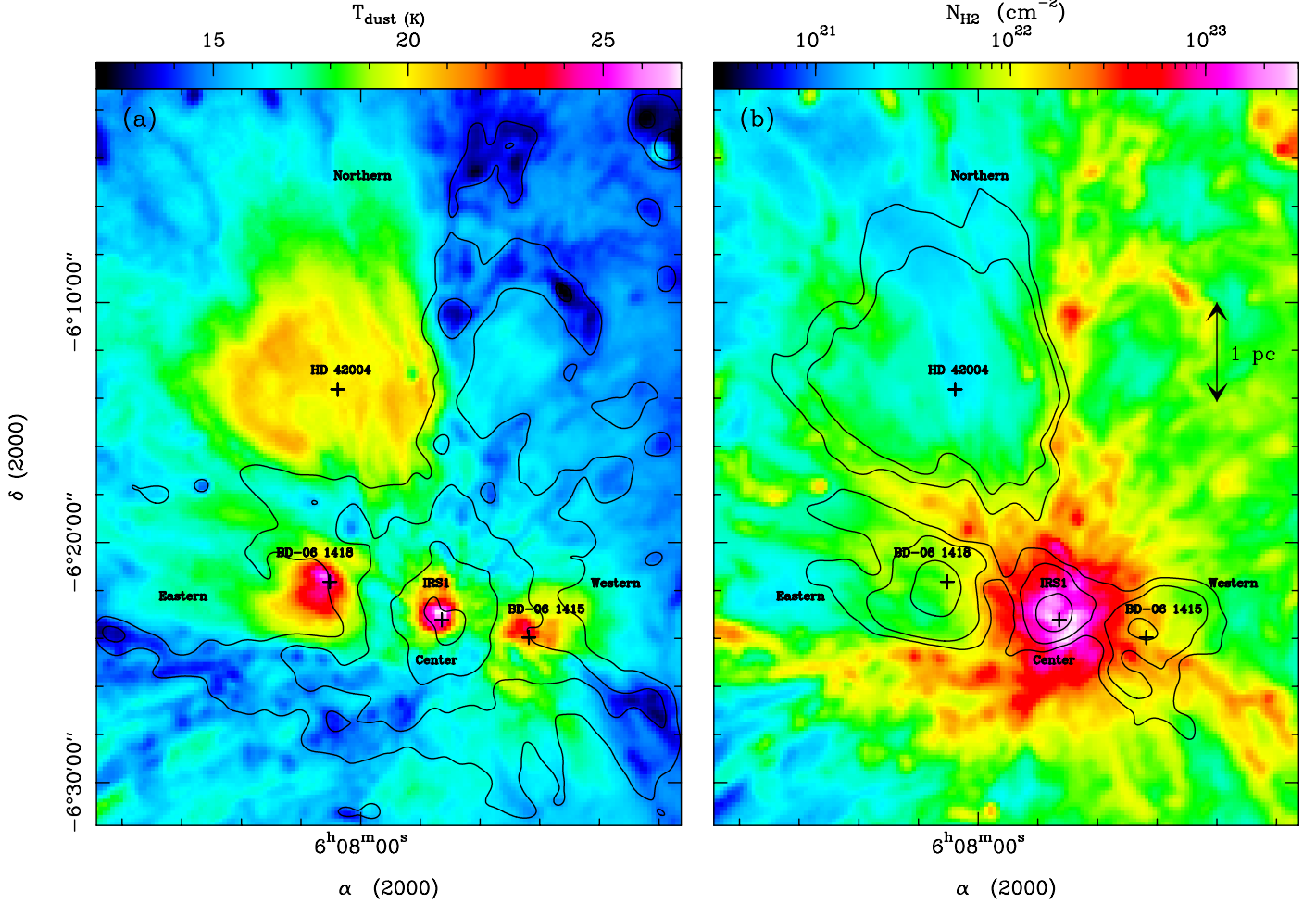
Fig. 2. Dust temperature (colours in a ) and contours in b ) and column density (colours in b ) and contours in a ) maps of the central part of the Mon R2 molecular cloud complex, covering the central, western, eastern, and northern H II regions with 36'' resolution. The heating sources of H II regions are indicated by a cross and with their name taken from Racine (1968) and Downes et al. (1975) . Smoothed temperature and column density contours are 17.5, 18.5, and 21.5 K and 7 \times 10^{21} , 1.5 \times 10^{22} , 5 \times 10^{22} , and 1.8 \times 10^{23} \text{ cm}^{-2} .
