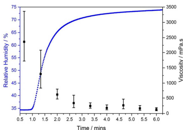
Fig. 6 Change in viscosity for a single salbutamol sulphate/NaCl/Cy3 aerosol (black squares) during an increase in RH from 34 to 74 % (blue line). Error bars are the standard deviations of the spread of the lifetimes within each FLIM image.
