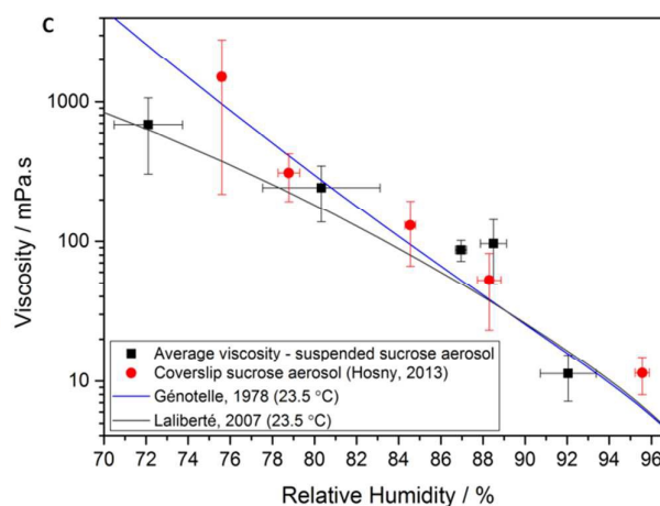
Fig. 4 (A) Example FLIM images for sucrose/Cy3 particles at different RHs (93, 88, 76 and 70%). (B) Fluorescence lifetime histograms for each image, representing the spread in the lifetimes across the image. An arbitrary colour scale has been assigned to the histograms and the images to label lifetime. (C) Change in viscosity of sucrose with RH. Black squares: Average change in viscosity with RH for suspended sucrose/Cy3 aerosol \pm standard deviation. Red circles: Average change in viscosity with RH for coverslip sucrose/Cy3 droplets \pm standard deviation. 27 Grey line: Calculated change in sucrose viscosity with RH using Laliberté's sucrose viscosity parameterisation. Blue line: Calculated change in sucrose viscosity with RH using Génotelle's empirical equation for sucrose viscosity as a function of water content. Sucrose models set at 23.5 °C.
