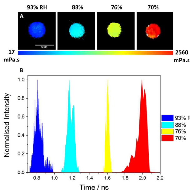
Fig. 4 (A) Example FLIM images for sucrose/Cy3 particles at different RHs (93, 88, 76 and 70%). (B) Fluorescence lifetime histograms for each image, representing the spread in the lifetimes across the image. An arbitrary colour scale has been assigned to the histograms and the images to label lifetime. (C) Change in viscosity of sucrose with RH. Black squares: Average change in viscosity with RH for suspended sucrose/Cy3 aerosol \pm standard deviation. Red circles: Average change in viscosity with RH for coverslip sucrose/Cy3 droplets \pm standard deviation. 27 Grey line: Calculated change in sucrose viscosity with RH using Laliberté's sucrose viscosity parameterisation. Blue line: Calculated change in sucrose viscosity with RH using Génotelle's empirical equation for sucrose viscosity as a function of water content. Sucrose models set at 23.5 °C.
