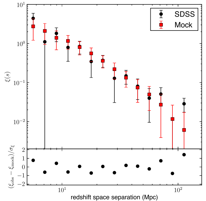
Figure 6. The two-point correlation function of SDSS-QSO DR7 and mean correlation function of the mock quasar catalogues. The error bars for SDSS quasars and mocks are the standard deviation from the correlation function computed using all the mocks, therefore including both Poisson or shot noise and cosmic variance. The lower panel shows the standardized residuals (difference between mock and observed correlation functions in each bin divided by the pooled standard error in the mocks \sigma_\xi ). All residuals are within two standard errors, indicating that both samples are statistically consistent with the same population hypothesis at 95 per cent confidence level.
