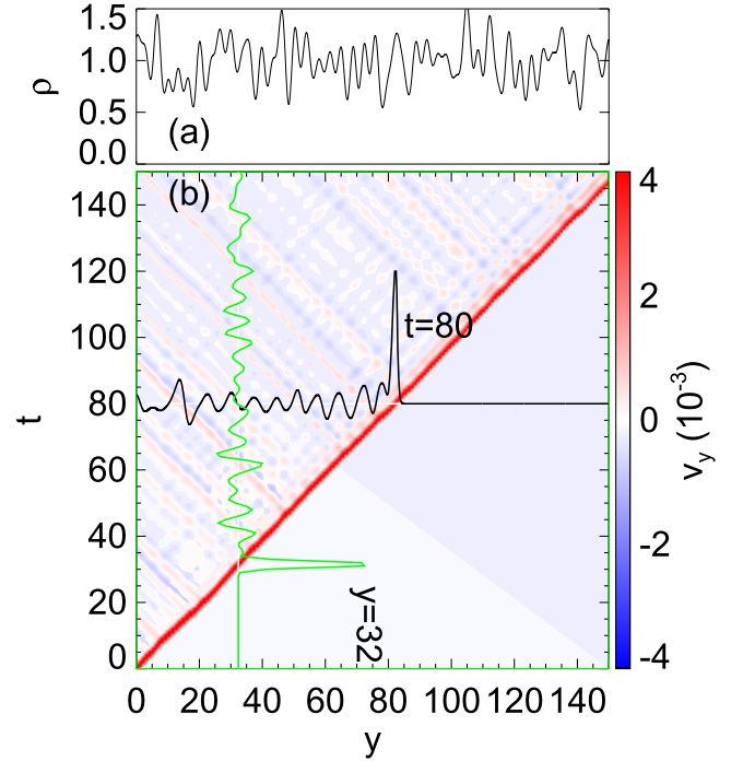
Figure 1. (a) Density distribution of a randomly structured plasma with a density contrast \delta_\rho = 0.18 and a correlation length L_c = 1.26 . (b) Distribution in the y - t plane of the y -component of the velocity perturbation ( v_y ) in response to a small-amplitude fast pulse with w_0 = 1.78 . The green (black) curve shows the temporal (spatial) distribution of v_y at y = 32 ( t = 80 ). In both curves, the values of v_y are multiplied by 10^4 for presentation purposes.
