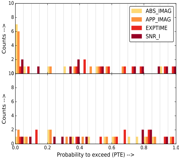
Figure 14. The distribution of the PTE values for four null tests before (top) and after (bottom) the SNR_{CON} cut. The peak near PTE value of zero in the top panel is because of (high \chi^2_{null} values) the deviation of the ratio of \partial N^{2796}/\partial z in the two subsets ( \mathcal{R}_{12} ) from unity. The PTE distribution looks uniform after ignoring the quasar spectra with poor SNR. This indicates that the null tests are successful and the absence of selection bias in the catalogue.
