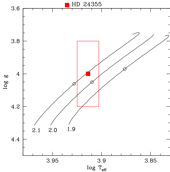
Figure 18. The \log T_{\text{eff}} - \log g diagram showing the spectroscopic parameter ( T_{\text{eff}}, \log g ) = (8200 \pm 200, 4.0 \pm 0.2) of HD 24355 and evolutionary tracks of 1.9, 2.0 and 2.1 M_{\odot} with a composition of (X, Z) = (0.70, 0.02) . The open circle along each track indicates the model that can reproduce the amplitude and the phase modulations of HD 24355.
