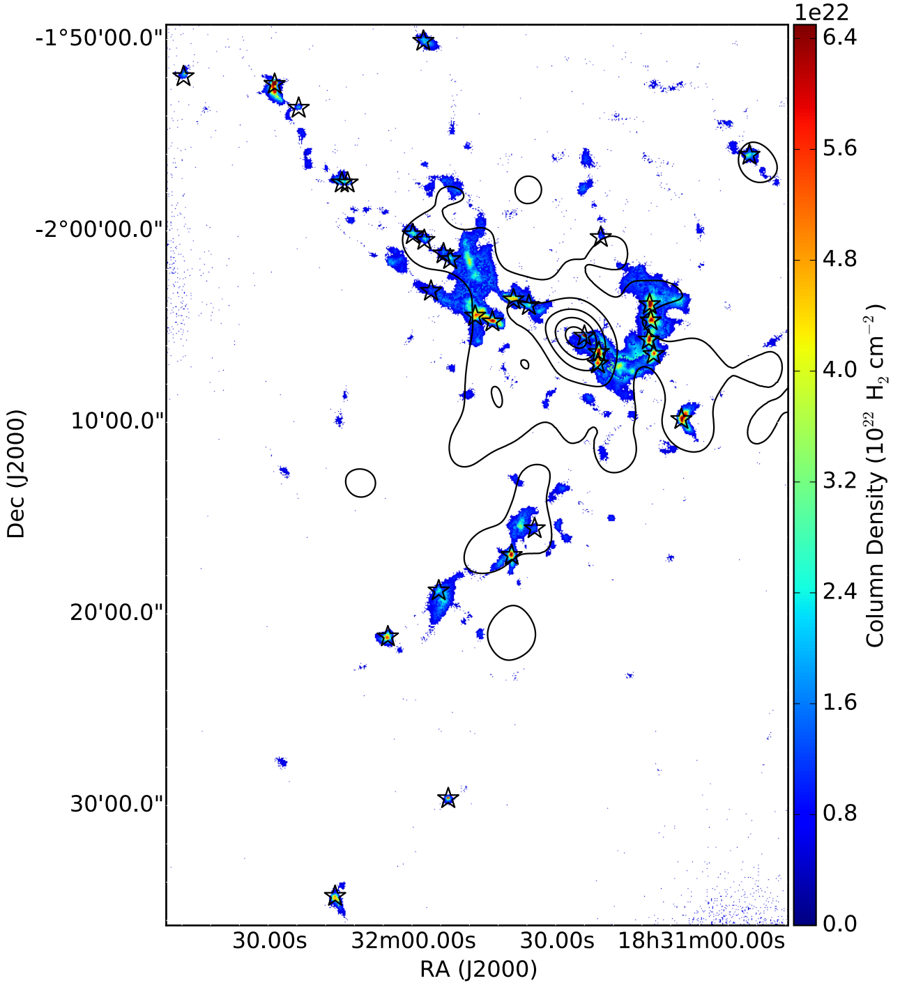
Figure 17. SCUBA-2 column density map of the W40 complex. Column density is shown for areas where emission is detected at or above S/N = 3 at 850\mu\text{m} . Column density is calculated using temperatures as presented in Figure 10 where available and a constant value of 15 K where a derived temperature is not. Contours describe YSO surface density with levels at 20, 60, 110, 160 and 210 YSO \text{pc}^2 . Stars mark the location of each dense core identified in Table 7.
