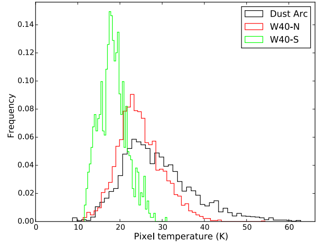
Figure 12. The normalised distribution of pixel temperatures across the W40 complex clouds: Dust Arc (black, warmest), W40-N (red) and W40-S (green, coolest).
