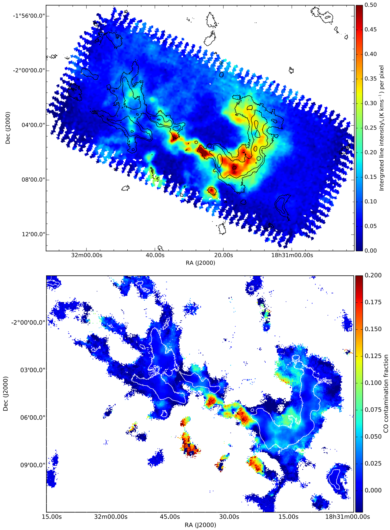
Figure 3. Upper ^{12}\text{CO} 3-2 integrated intensity map over the entire range (from -90 to +100 km s ^{-1} ) of the central region of the W40 complex. Contours show SCUBA-2 850 \mu\text{m} emission at the 5 \sigma , 15 \sigma and 50 \sigma levels. Lower the fraction of SCUBA-2 850 \mu\text{m} that can be attributed to ^{12}\text{CO} 3-2 345 GHz line emission. The SCUBA-2 data are masked at 3 \sigma and the 5 \sigma level is shown by the white contour.
