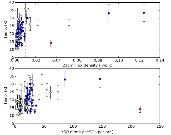
Figure 16. Clump temperature as a function of: (upper) mean VLA 21 cm flux detected in the area of each clump; and (lower) YSO surface density. In both plots, filled markers represent protostellar clumps whereas hollow markers represent starless clumps. W40-SMM 19 is considered anomalous and its data are flagged as a red point. Red lines mark the partition between clump temperature regimes.
