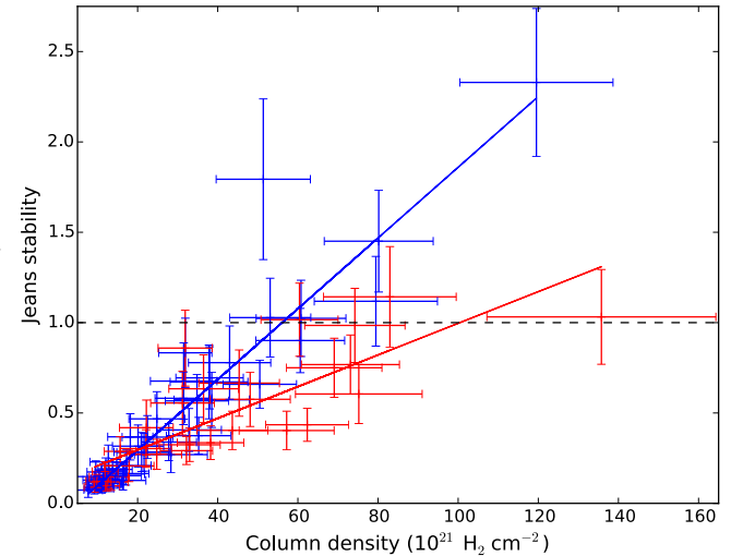
Figure 19. Jeans stability, M_{850}/M_J , as a function of column density. Exterior peripheral clumps (defined as having a mean Herschel 70 \mu\text{m} flux of less than 1000 MJy/Sr) are marked in blue, interior clumps within the nebulosity Sh2-64 are marked in red. The unweighted linear regression fit to each population is marked as a line of the same colour.
