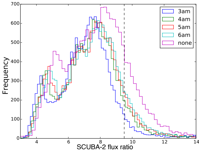
Figure C1. Histograms of flux ratio for the Aquila CO subtracted SCUBA-2 reductions with varying spatial filters applied. Filter sizes, in arcminutes, are labelled on the plot. The flux ratios calculated with no filter are also included for comparison. Histograms are examined for total volume below 9.5, an arbitrary value above which ratios are considered unphysical.
