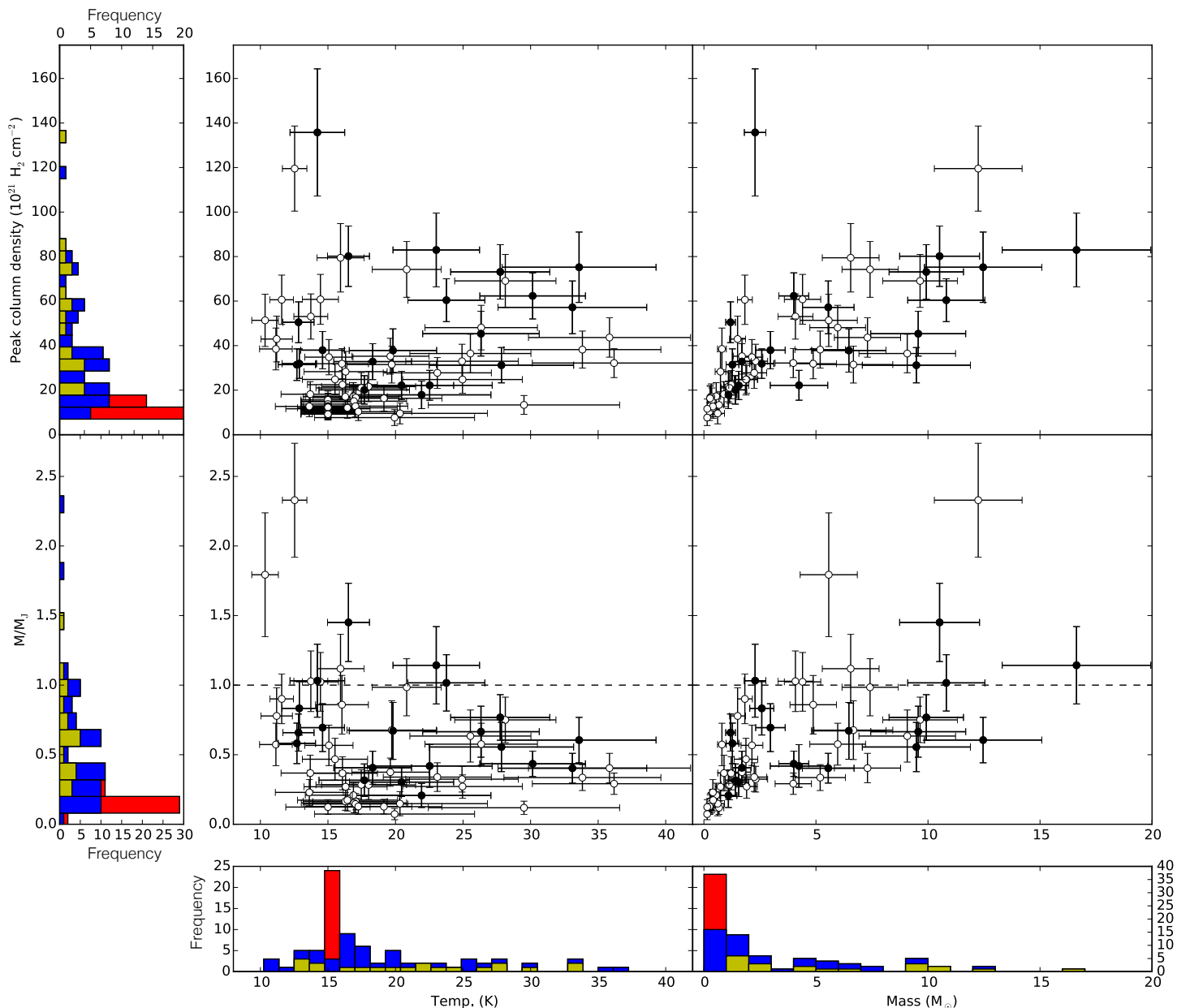
Figure 14. Properties of clumps within the W40 complex. Histograms show the distribution of mass, temperature, M/M_J and peak column density. Total height of each bar represents the total number of clumps in each bin whereas each colour represents a specific subset: blue for clumps that have measured temperature, yellow for clumps with measured temperatures that contain at least one YSO, and red for clumps with no temperature data, for which the value 15 \pm 2 K is assumed. Scatter plots show any existing correlation between clump properties: top left shows column density as a function of temperature, top right shows column density as a function of mass, bottom left shows Jeans stability, M_{850}/M_J , as a function of temperature and bottom right shows Jeans stability as a function of mass. Filled markers indicate protostellar clumps and hollow markers indicate starless clumps.
