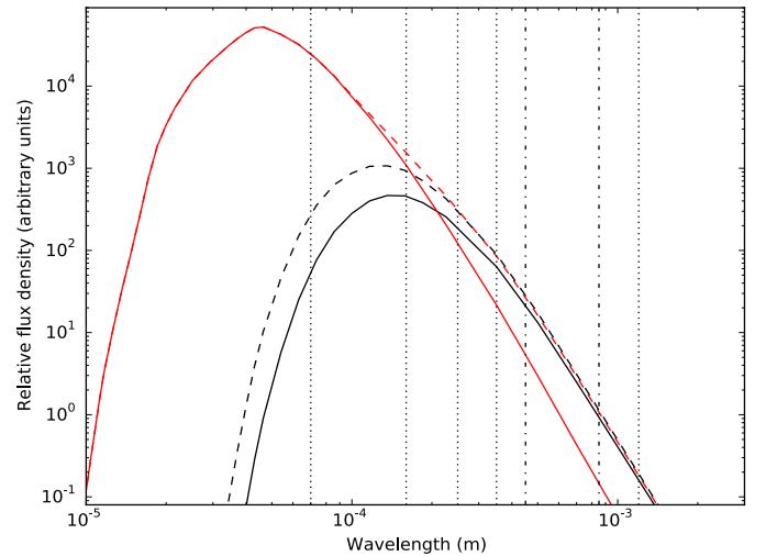
Figure E1. Model opacity-modified blackbody SEDs for a cold (black, 15\text{ K} ) cloud and a hot (grey, red online, 50\text{ K} ) cloud with 3% of the mass of the cold cloud. The red dashed SED represents the two cloud components combined and the black dashed SED represents how the combined SED resembles a single 17\text{ K} cloud at SCUBA-2 450 and 850\mu\text{m} bands (dot-dashed vertical lines). The Herschel 70 , 160 , 250 and 350\mu\text{m} bands, and the MAMBO 1.2\text{ mm} band are also marked (dotted vertical lines). Note how the 50\text{ K} component dominates the fluxes at 70 and 160\mu\text{m} .
