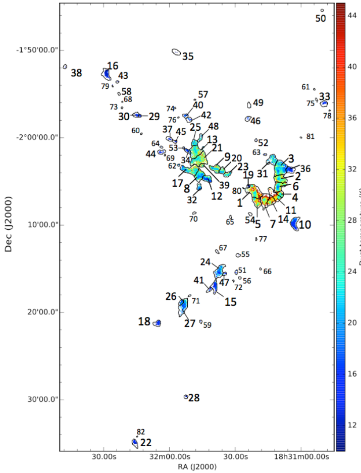
Figure 13. Temperature map of the W40 complex with clumps identified in the SCUBA-2 CO subtracted, 4' filtered, and free-free subtracted 850 \mu\text{m} data using the Starlink clump-finding algorithm FELLWALKER plotted as contours. Clumps are indexed in order of highest to lowest flux density, matching the order presented in Tables 5 and 6.
