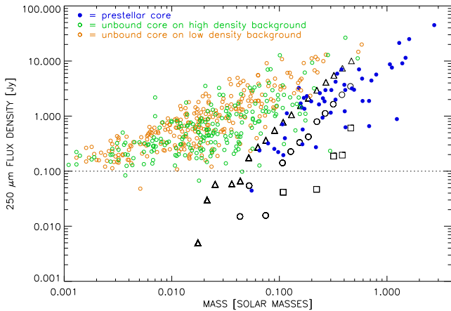
Figure A1. The 250\ \mu\text{m} flux densities of observed and model cores as a function of mass. Black symbols represent the model prestellar cores used in the completeness simulation, taken to be critical BE spheres. They are plotted for three density regimes, indicated by triangles (low-density case), open circles (moderate-density case) and squares (high-density case). Also shown for comparison are the observational values for the extracted sources, represented by the coloured symbols. These are divided into prestellar cores (blue filled circles), and gravitationally unbound cores (open circles, where green and gold designate those seen against high and low column density backgrounds, respectively, based on a threshold of A_V = 7 mag). For reference, the horizontal dotted line represents the approximate flux density sensitivity limit.
