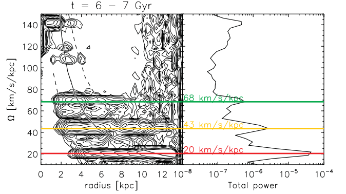
Figure 4. Left: power spectrum of m = 2 frequencies as a function of radius in the disc, for the time interval 6–7 Gyr. The solid black line marks \Omega_c , while the dashed black lines mark \Omega_c \pm \kappa/2 . The three main spiral patterns are identified by coloured horizontal lines. Right: the global frequency spectrum. Contour levels vary in logarithm from 5 \times 10^{-10} to 1 \times 10^{-6} .
