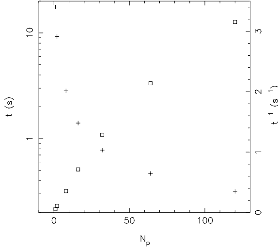
Figure 2. The performance of our implementation of \chi^2\text{M2M} . We used 1.8 \times 10^6 particles without potential calculations or particle motion. On the left-hand axis, we label time per step required, with the corresponding data indicated by plus symbols, while on the right-hand axis we label steps per unit time, with the corresponding data now shown by the open squares. Note that the scale is logarithmic on the left-hand side and linear on the right-hand side. The fraction of sequential code, f , from these data was computed at \sim 1 per cent.
