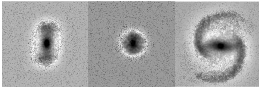
Figure 7. Three different final states of the harassed galaxies (unsharp nosified images). From left to right: bar-like galaxy (GAL7 of Table 1), spherical spheroid (GAL6) and spiral galaxy (GAL3). The addition of noises often hides ring structures surrounding the central bar, which is the case of the first remnant on the left. In order to point out the characteristic structure of the remnants we used two physical scales: the two images on the left have a box side of \sim 12 kpc, while the box size of the spiral galaxy on the right is \sim 30 kpc.
