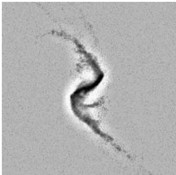
Figure 8. Tidal tails of GAL6 (Table 1) generated during a pericentric passage (unsharp nosified image). These smooth features are visible only for a short time (typically about 0.2–0.3 Gyr) since they are heated and evaporated by continued encounters with cluster substructures.
