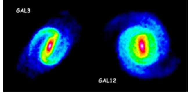
Figure 14. Surface density distribution of the two remnants presenting a nearly face-on spiral pattern. The physical size of both the images is \sim 12 \text{ kpc} .
