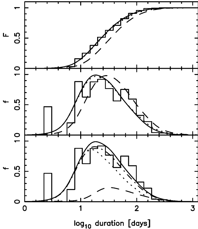
FIG. 1.—ETD of the COBE-Dyn model compared to the detection-efficiency-corrected observations of the MACHO group (histograms in all panels). Top : Cumulative distribution function for the standard model, (M_L^c, M_L^r) = (0.04, 4) (solid line), the best model with (M_L^c, M_L^r) = (0.04, 10) (dotted line), and a model with (M_L^c, M_L^r) = (0.075, 10) (dashed line). We obtain D_{KS} = 0.081, 0.068, 0.213 , respectively, for the three models. Middle : Differential distributions of these models (same line styles). (In these two panels, all model distributions have been smoothed with a kernel density estimator of bandwidth 0.1.) Bottom : ETD of the (M_L^c, M_L^r) = (0.04, 4) model and its decomposition into events with 6 \leq D_s \leq 10 kpc (dotted line), 0 \leq D_L \leq 4 kpc (dashed line), and D_L > 4 kpc (dot-dashed line).
