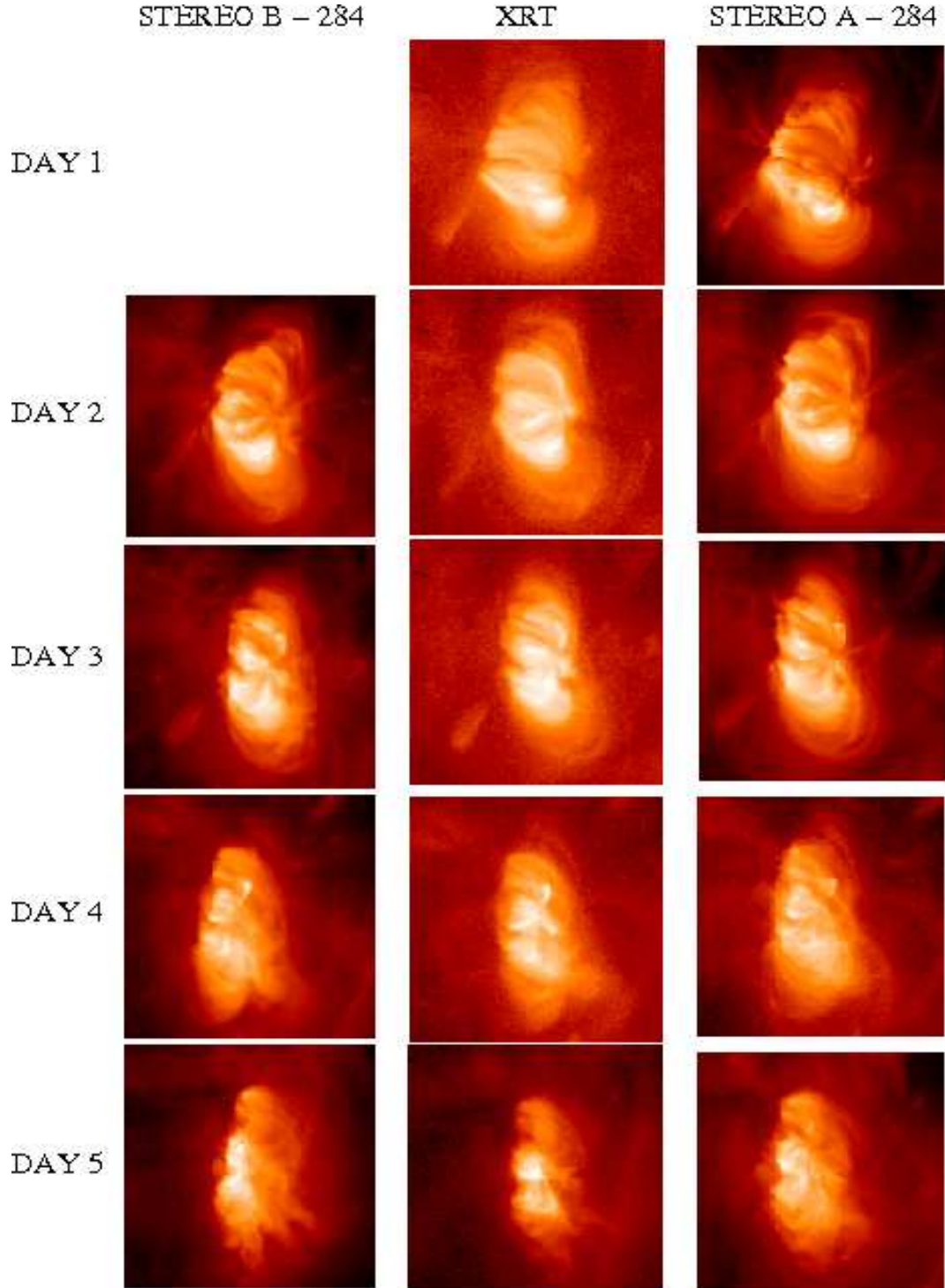
Fig. 9.— Left: STEREO B EUVI 284 Å images taken at \sim 12:30 UT for each day (apart from Day 1) of the observing run. Middle: Hinode XRT images taken at approximately the same time as the EUVI images. Right: STEREO A EUVI 284 Å images taken at \sim 12:30 UT for each day of the observing run.
