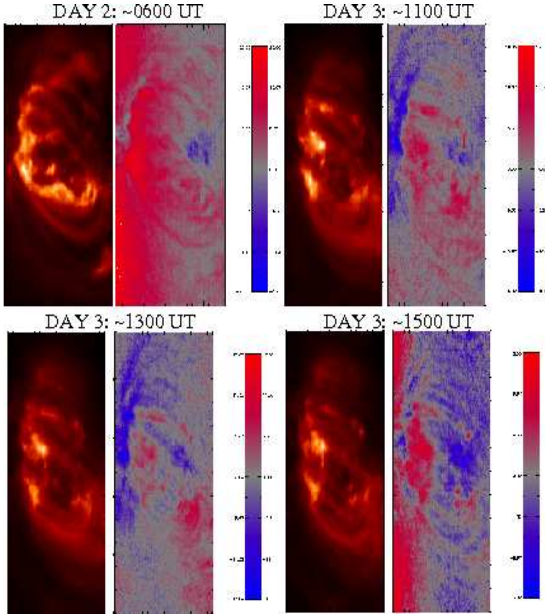
Fig. 14.— Velocity maps from EIS data for Days 2 & 3 presented alongside their intensity images for Fe XII. The strong intensities also represent the high density regions.
