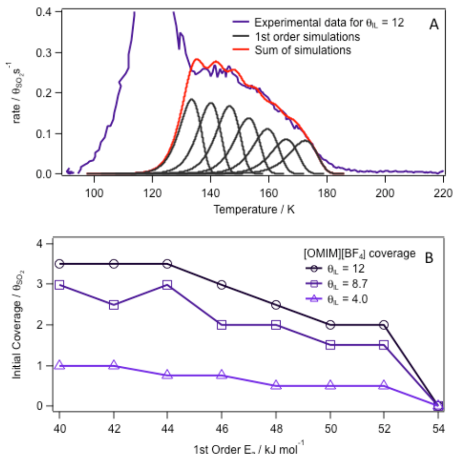
Figure 8. A, TPD of IL ( \theta_{IL} = 12 ) co-adsorbed with SO_2 ( \theta_{SO_2} = 50 \pm 4 ) fitted with the sum of seven first order TPD curves. B, initial coverages versus first order activation energies for the simulated fits to the desorption curve for \theta_{IL} = 4, 8.7, \text{ and } 12 when co-adsorbed with, \theta_{SO_2} = 50 \pm 4 in the range to 130 \text{ K} < T < 180 \text{ K} .
