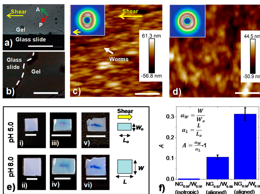
Figure 3. POM images of DX NG 0.5 /W 0.5 gels prepared using (a) linear shear and (b) without shear. A and P in (a) are the directions of the analyzer and polarizer. (c, d) AFM images obtained for anisotropic and isotropic DX NG 0.5 /W 0.5 composites in water, respectively. 2D SAXS patterns for each film are shown as insets. The shear direction for the inset in (c) is indicated. (e) Isotropic DX NG 0.5 /W 0.5 (i, ii), anisotropic DX NG 0.92 /W 0.08 films (iii, iv), and anisotropic DX NG 0.5 /W 0.5 (v, vi) films at pH 5.0 or 8.0. Blue marker pen lines were used to record the shear directions. Scale bars: (a, b) 400 \mu m; (c, d) 200 nm; (e) 6.0 mm. The cartoon depicts the anisotropic swelling. (f) Anisotropic swelling parameters ( A ) from the images shown in (e).
