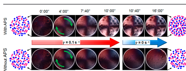
Figure 2. Rotational shear ( \gamma ) was applied to NG_{0.5}/W_{0.5} binary mixtures while being viewed with polarized light using SIPLI. The samples were heated to 45^\circ\text{C} , and the shear was terminated after 10 min. The top row shows the sample that underwent double cross-linking (and formed DX NG_{0.5}/W_{0.5} ) during shear due to APS. The bottom row shows the control sample that did not contain APS. The green arrows indicate the direction of shear, and the cartoons depict the proposed initial and final composite gel morphologies.
