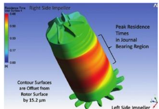
Figure 19. Peak residence times in journal bearing region. (Source [75])
