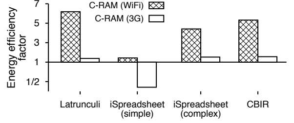
Fig. 10: Effect of C-RAM on device energy consumption
