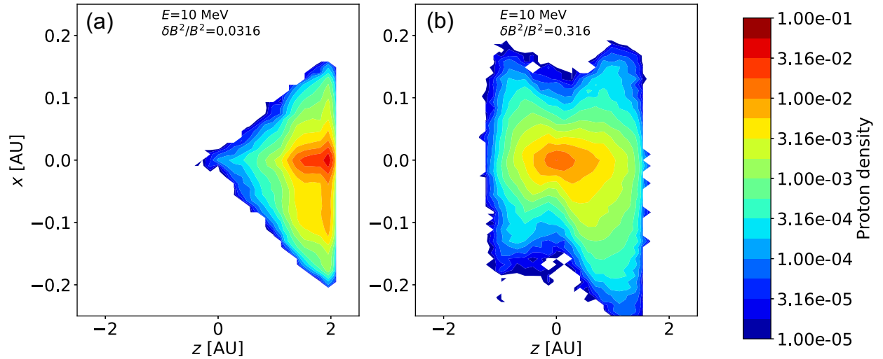
Figure 3. Contours of the spatial distributions of 10 MeV protons with turbulence amplitudes 0.0316 and 0.316, and q_{\parallel} = 5/3 . The contours are given at the times when the times when an unscattered proton of the given energy would have propagated a distance of 2 au, at t = 2.04 h.
