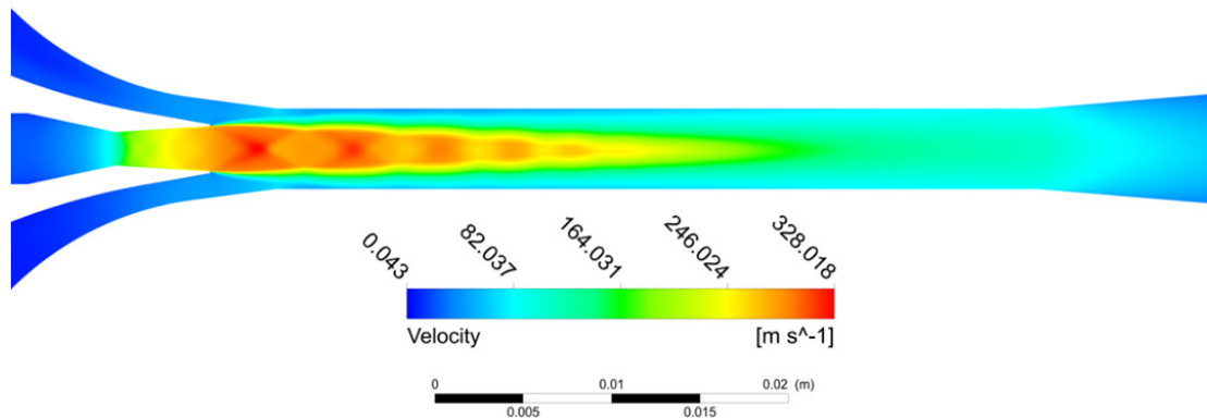
Fig. 3. CFD model of the ejector.
