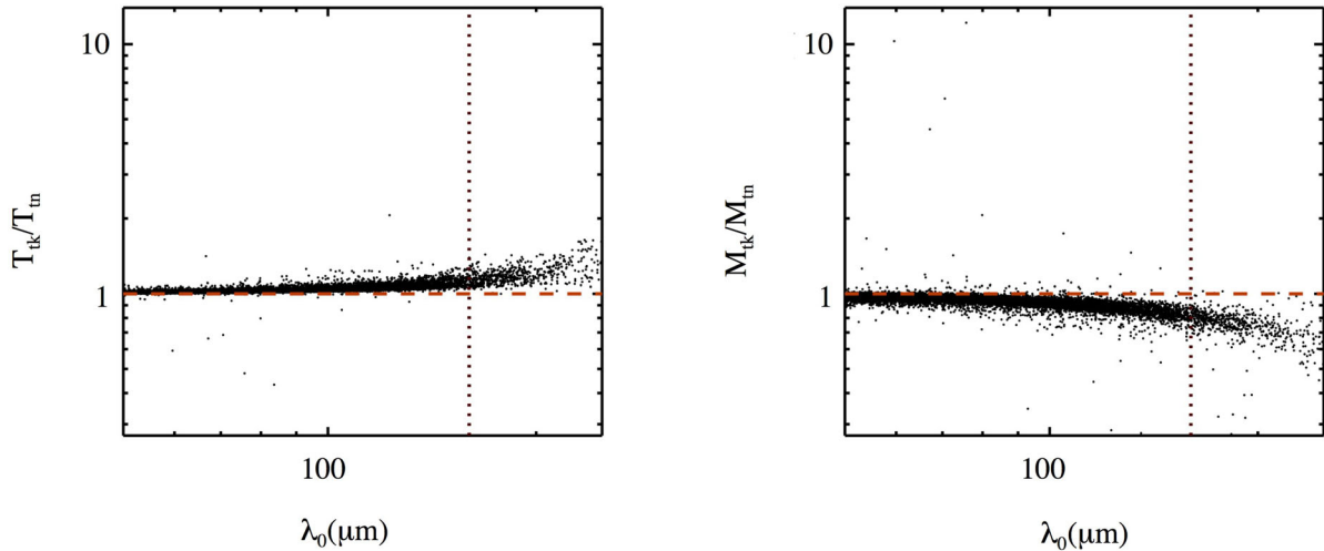
Figure 3. Left-hand panel: ratio of the dust temperatures derived by fitting equations (1) and (4) to SEDs (and denoted here with T_{ik} and T_{in} , to indicate an optically ‘thick’ and ‘thin’ regime, respectively) versus the corresponding \lambda_0 obtained through equation (1). The x -axis starts from 50.6 \mu\text{m} , corresponding to the minimum value for which this comparison makes sense (see text). The \lambda_0 = 160 \mu\text{m} value is highlighted as a reference with a vertical dotted line. The red dashed line represents the T_{ik} = T_{in} condition. Right-hand panel: the same as the left-hand panel, but for the masses M_{ik} and M_{in} derived through equations (3) and (4), respectively.
