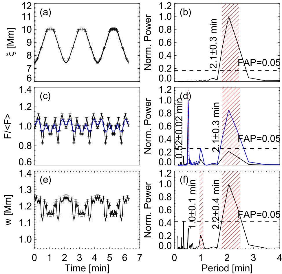
Figure 11. Same as Figure 10, but for Model V. In panel (c), the blue continuous line plots the four-point running average of normalized flux; and the power spectrum (blue line) has enhanced peaks in long-period range.
