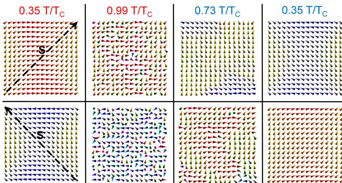
Figure 4. Magnetisation switching simulations. Snapshots of the magnetisation configuration are shown at different temperatures, illustrating the switching process. The top row starts from state “1” with a stress applied to induce switching to state “0”. The bottom row starts from state “0” and switches to state “1”.
