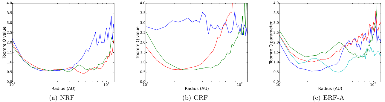
Figure 5. As per Fig. 3, for Toomre Q radial distribution.
