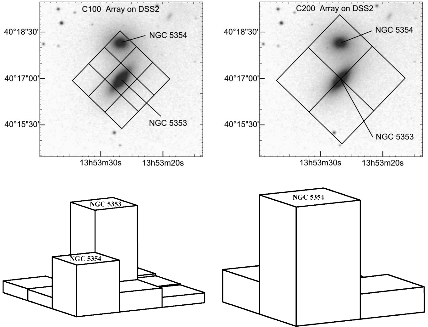
FIG. 1.—Infrared Digitized Sky Survey 2 images of NGC 5353 and NGC 5354 with superposed ISOPHOT C100 (top left) and C200 (top right) array pointings that were used for the ISO observations of these galaxies. Bottom left and right: Three-dimensional histograms of the ISO 100 and 180 \mu\text{m} fluxes, respectively, before the individual galaxy fluxes were corrected for aperture size (see text). For visual clarity, the histograms are oriented so that the fainter source is plotted in the foreground.
