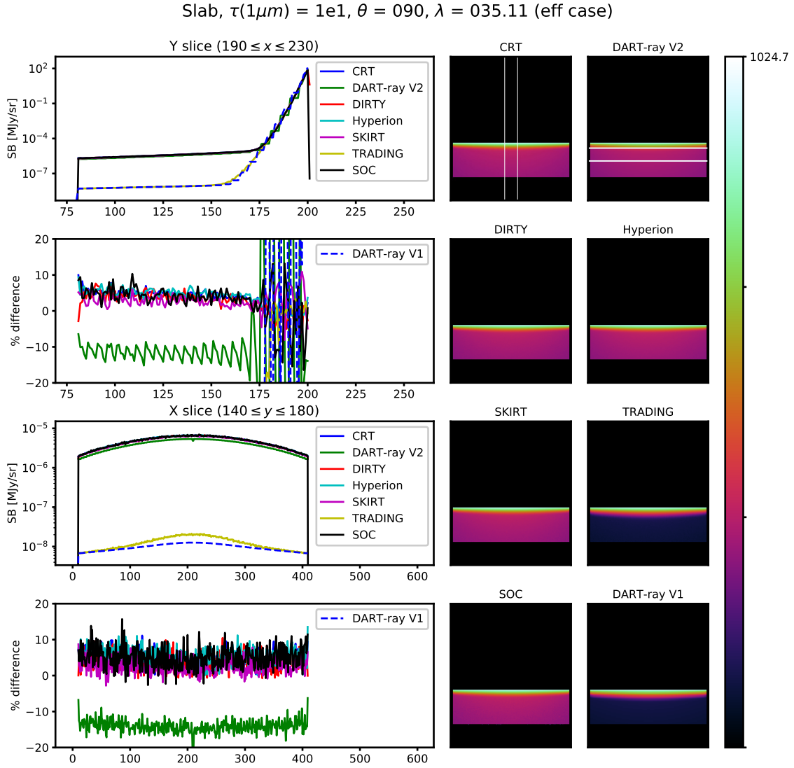
Fig. 4. Comparison of the \lambda = 35.11 \mu m edge-on images of the TRUST slab benchmark for the vertical optical depth \tau(1 \mu m) = 10 . The solutions provided by the old and new DART-Ray version are included as well as those of the other codes participating to the project. Units on the images are MJy/sr. The plots on the left show the average surface brightness profiles and the relative differences between the solutions along a vertical and a horizontal strip, whose boundaries are shown within the top two images (CRT and new DART-Ray code). The X-axis of these plots are in units of pixels. The inclusion of dust self-heating in the new version of DART-Ray allows a much closer agreement with the other codes. We note that these solutions are for the “effective grain” case (see G17).
