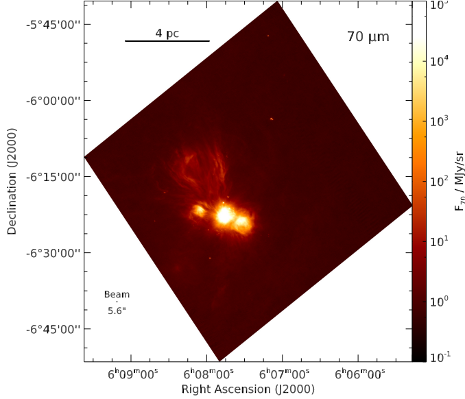
Fig. A.1. Monoceros R2 as viewed by Herschel PACS 70\,\mu\text{m} . The image is 1.15^\circ \times 1.3^\circ ( 16.7 \times 19.1\,\text{pc} ) in size. The diffraction-limited instrumental beam ( 5.6'' ) is shown to the lower left of the image.
