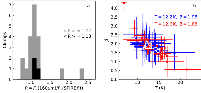
Fig. 7. Comparison of Herschel MBB fits with and without the 160\,\mu\text{m} data point in the case of the P(\chi^2)=25\% clump sample with \theta_{\text{F}} = 500'' and LM masks. The left frame shows the distribution of ratios between the 160\,\mu\text{m} flux density and the value predicted by the 250\text{--}500\,\mu\text{m} fit. The grey histogram contains all clumps, and the black histogram is based on three clumps with YSO candidates. The second frame shows (T, \beta) values for individual clumps for the 250\text{--}500\,\mu\text{m} (blue triangles) and 160\text{--}500\,\mu\text{m} (red squares) fits. The circles indicate clumps with YSO candidates. The median values are quoted in the frame and are plotted with larger symbols.
